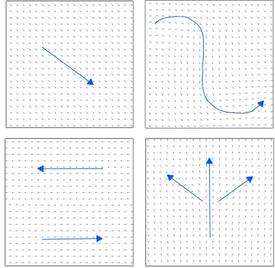
Figure 6: Examples of guide curves (shown in blue) and their resulting IFs. The gray arrows are the IF vectors (following from the interpolation scheme of Section 5.2.1) on a 20 \times 20 sample grid.
