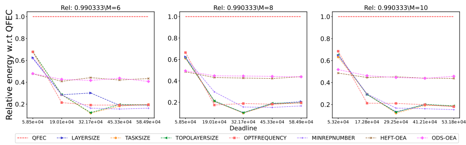
Figure 2890: Assessing the performance of different processor number on the SoyKB workflow.
