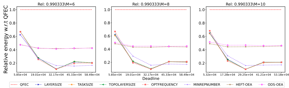
Figure 2868: Assessing the performance of different processor number on the SoyKB workflow.
