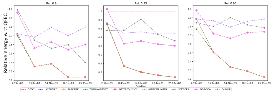
Figure 1760: Assessing the performance of EXTMILP on the SRASearch workflow (with 10 tasks).
