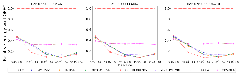
Figure 2659: Assessing the performance of different processor number on the SoyKB workflow.
