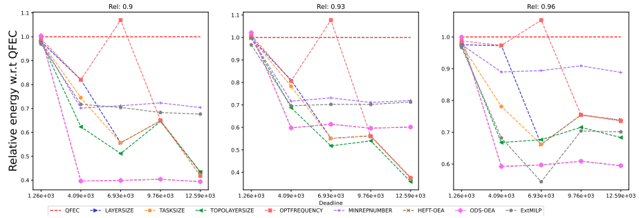
Figure 2090: Assessing the performance of EXTMILP on the Epigenomics workflow (with 20 tasks).
