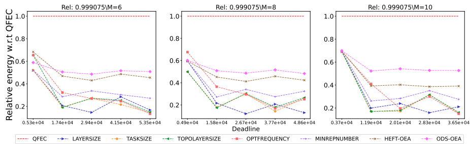
Figure 2862: Assessing the performance of different processor number on the Epigenomics workflow.
