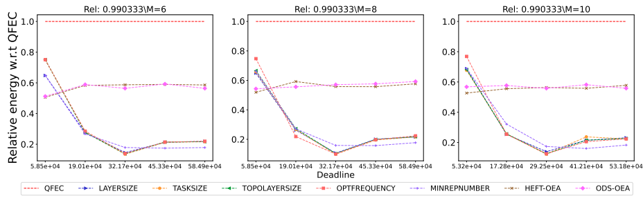
Figure 2560: Assessing the performance of different processor number on the SoyKB workflow.
