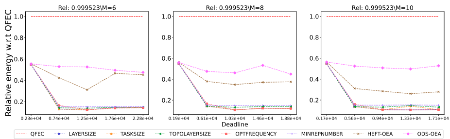
Figure 2529: Assessing the performance of different processor number on the BWA workflow.
