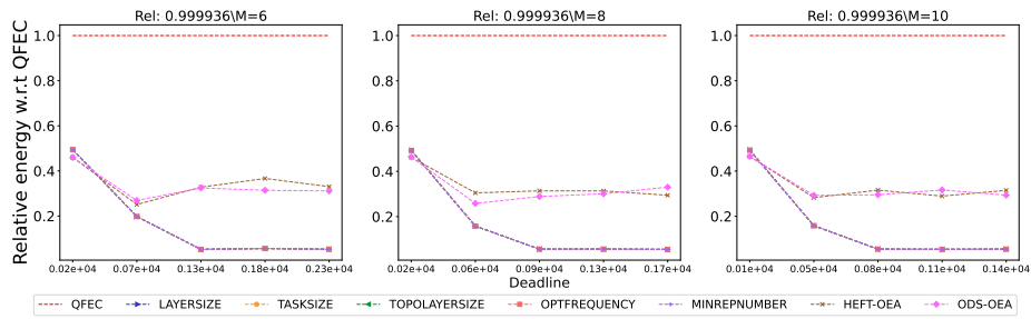
Figure 2658: Assessing the performance of different processor number on the Seismology workflow.
