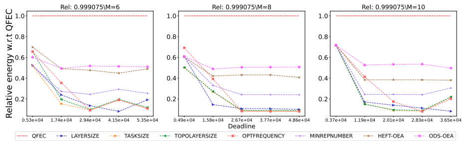
Figure 2466: Assessing the performance of different processor number on the Epigenomics workflow.
