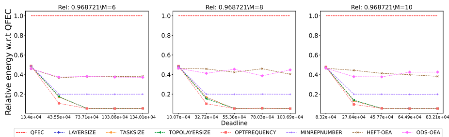
Figure 2781: Assessing the performance of different processor number on the BLAST workflow.
