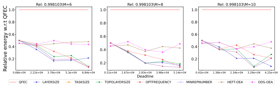
Figure 2481: Assessing the performance of different processor number on the QR.
