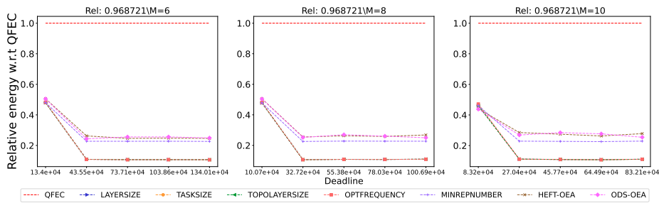
Figure 2660: Assessing the performance of different processor number on the BLAST workflow.
