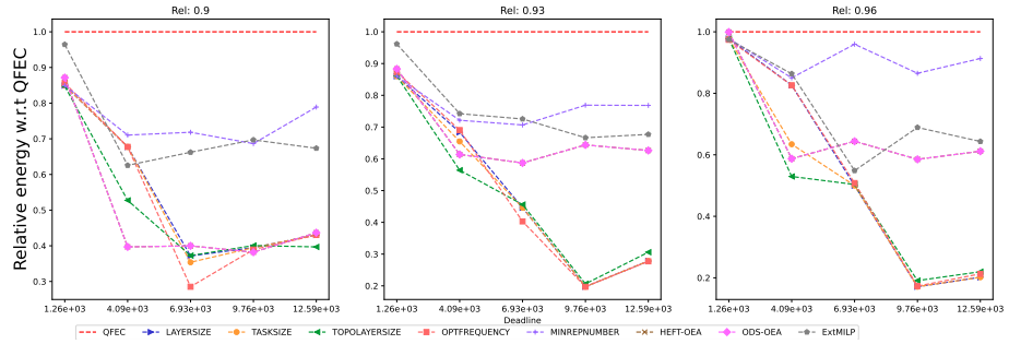
Figure 1610: Assessing the performance of EXTMILP on the Epigenomics workflow (with 20 tasks).
