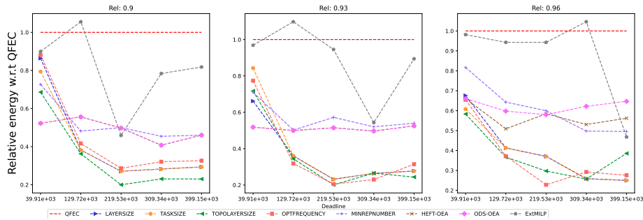
Figure 1579: Assessing the performance of EXTMLP on the SoyKB workflow (with 30 tasks).
