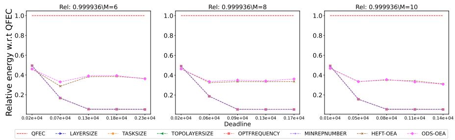
Figure 2702: Assessing the performance of different processor number on the Seismology workflow.
