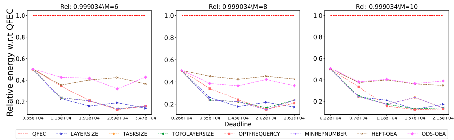
Figure 2805: Assessing the performance of different processor number on the Cholesky workflow.
