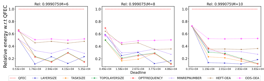
Figure 2532: Assessing the performance of different processor number on the Epigenomics workflow.
