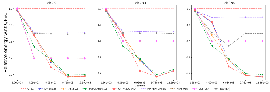
Figure 890: Assessing the performance of EXT MILP on the Epigenomics workflow (with 20 tasks).
