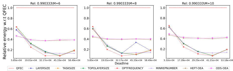
Figure 2835: Assessing the performance of different processor number on the SoyKB workflow.
