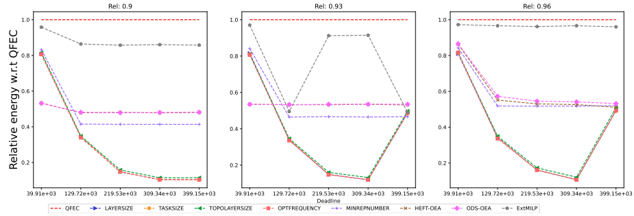
Figure 839: Assessing the performance of EXT MILP on the SoyKB workflow (with 30 tasks).
