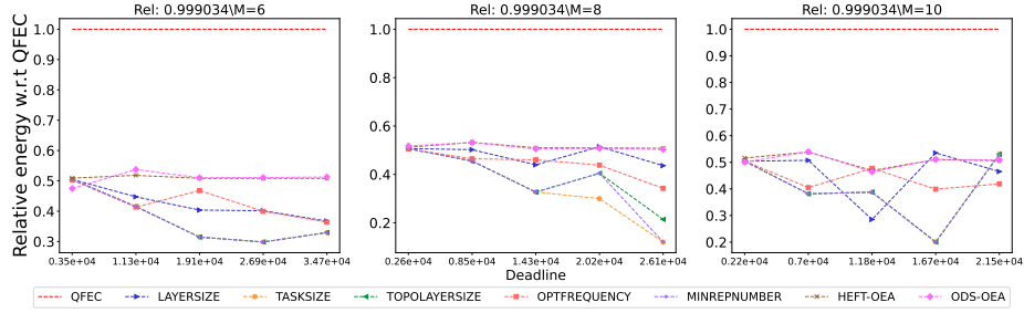
Figure 2563: Assessing the performance of different processor number on the Cholesky workflow.
