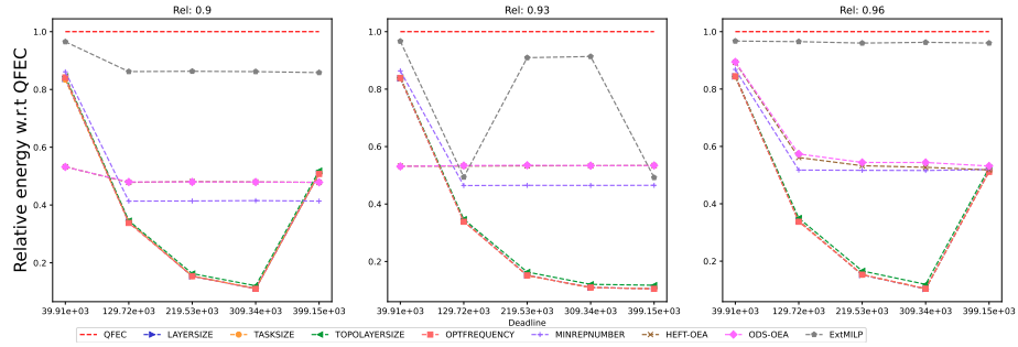
Figure 919: Assessing the performance of EXT MILP on the SoyKB workflow (with 30 tasks).
