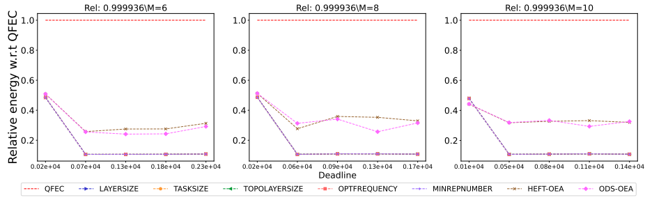
Figure 2724: Assessing the performance of different processor number on the Seismology workflow.
