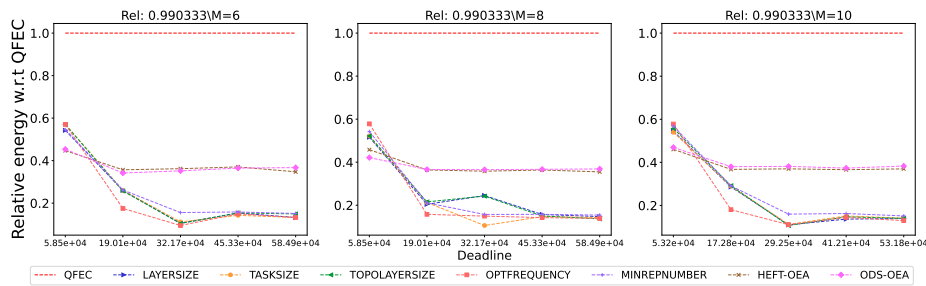
Figure 2758: Assessing the performance of different processor number on the SoyKB workflow.
