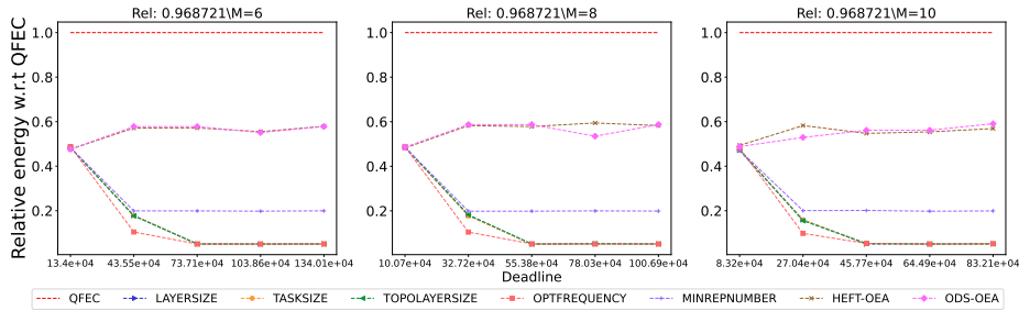
Figure 2517: Assessing the performance of different processor number on the BLAST workflow.
