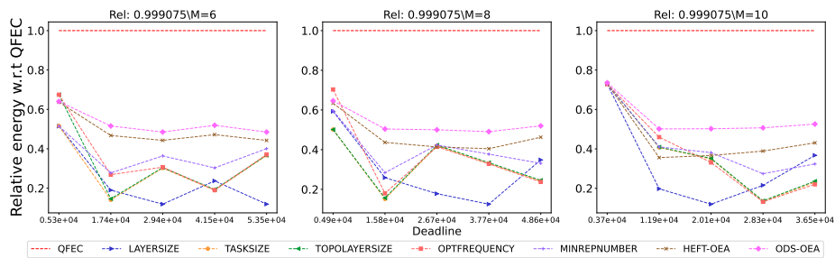
Figure 2587: Assessing the performance of different processor number on the Epigenomics workflow.
