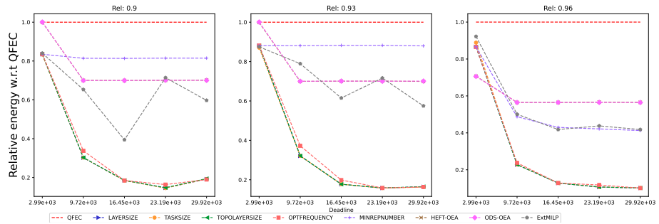
Figure 921: Assessing the performance of EXT MILP on the SRASearch workflow (with 20 tasks).
