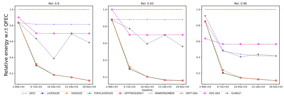
Figure 841: Assessing the performance of EXT MILP on the SRASearch workflow (with 20 tasks).
