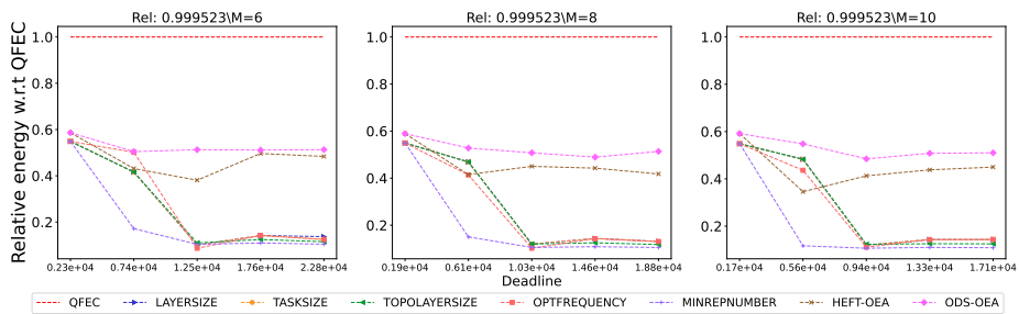
Figure 3002: Assessing the performance of different processor number on the BWA workflow.
