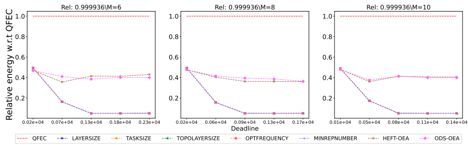
Figure 2394: Assessing the performance of different processor number on the Seismology workflow.
