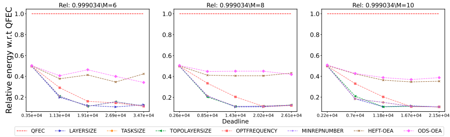
Figure 2398: Assessing the performance of different processor number on the Cholesky workflow.
