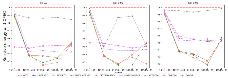
Figure 2039: Assessing the performance of EXTMILP on the SoyKB workflow (with 30 tasks).
