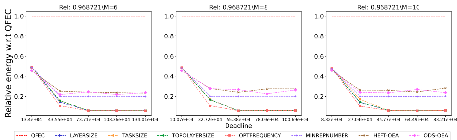
Figure 2649: Assessing the performance of different processor number on the BLAST workflow.
