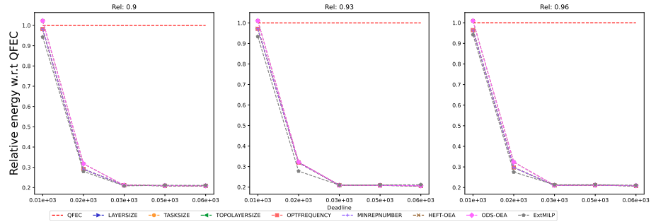
Figure 2056: Assessing the performance of EXTMILP on the Seismology workflow (with 20 tasks).
