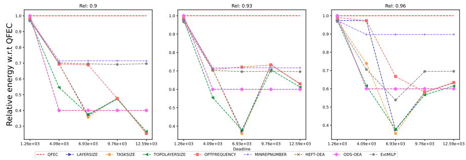
Figure 1290: Assessing the performance of EXTMILP on the Epigenomics workflow (with 20 tasks).
