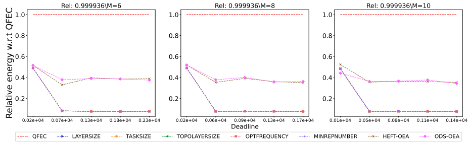
Figure 2779: Assessing the performance of different processor number on the Seismology workflow.
