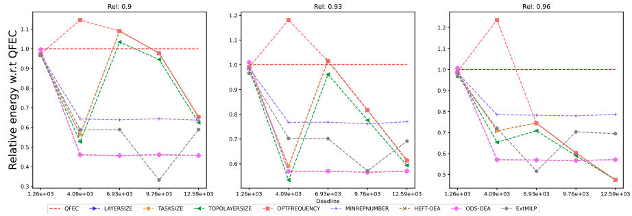
Figure 2210: Assessing the performance of EXTMILP on the Epigenomics workflow (with 20 tasks).
