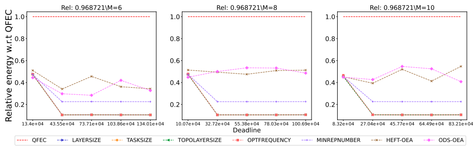
Figure 2440: Assessing the performance of different processor number on the BLAST workflow.
