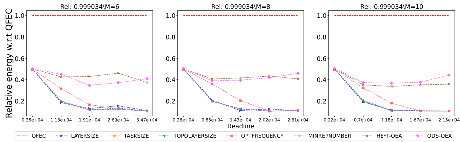
Figure 2409: Assessing the performance of different processor number on the Cholesky workflow.
