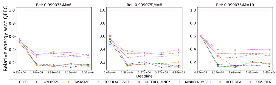
Figure 2675: Assessing the performance of different processor number on the Epigenomics workflow.
