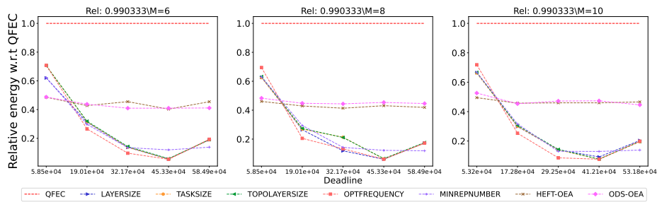
Figure 2483: Assessing the performance of different processor number on the SoyKB workflow.
