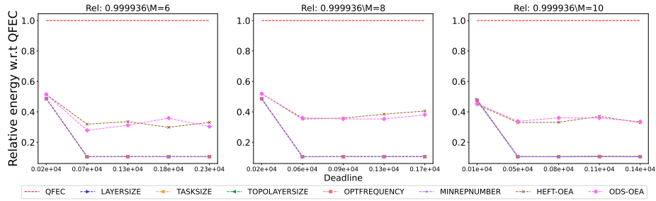
Figure 2372: Assessing the performance of different processor number on the Seismology workflow.
