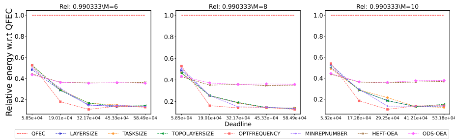
Figure 2725: Assessing the performance of different processor number on the SoyKB workflow.
