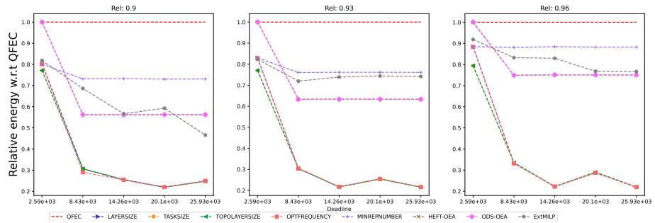
Figure 1120: Assessing the performance of ExtMILP on the SRASearch workflow (with 10 tasks).
