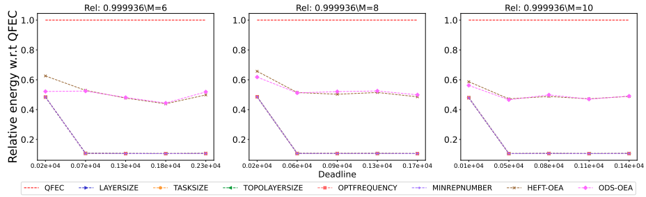
Figure 2581: Assessing the performance of different processor number on the Seismology workflow.
