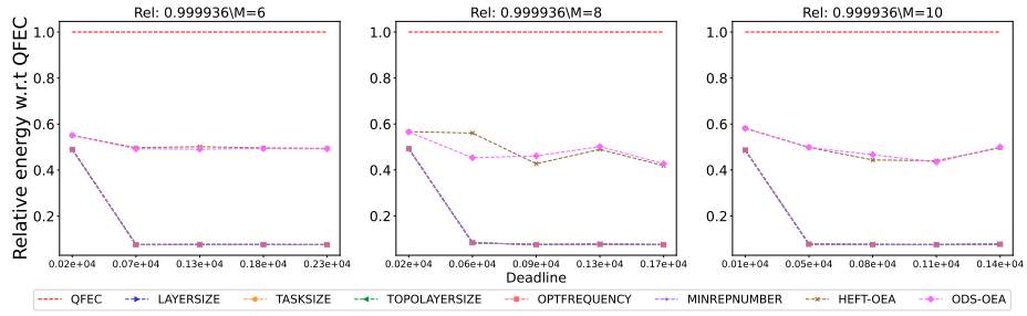
Figure 2559: Assessing the performance of different processor number on the Seismology workflow.
