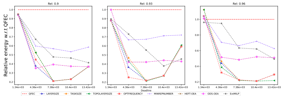
Figure 1583: Assessing the performance of EXT MILP on the BWA workflow (with 10 tasks).
