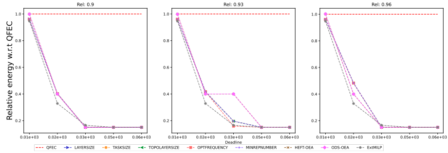
Figure 896: Assessing the performance of EXT MILP on the Seismology workflow (with 20 tasks).
