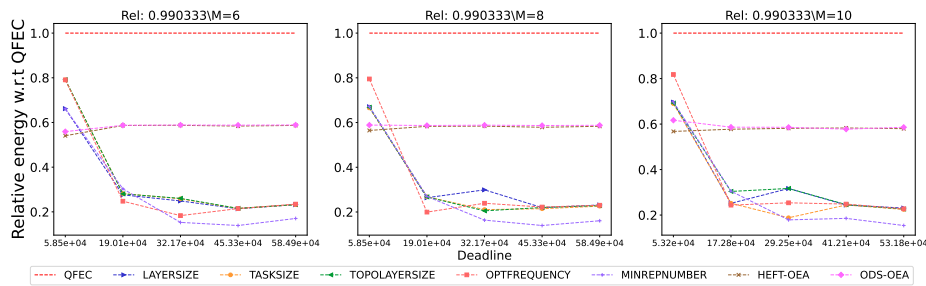
Figure 2637: Assessing the performance of different processor number on the SoyKB workflow.
