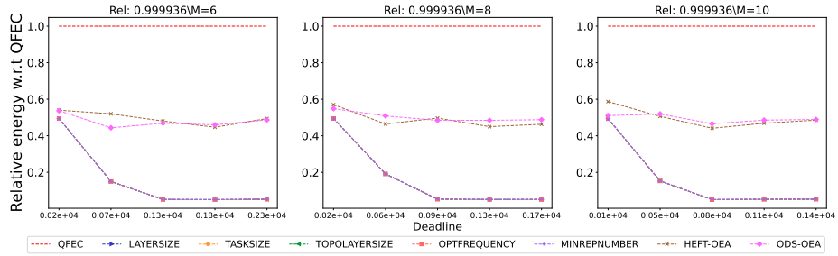
Figure 2570: Assessing the performance of different processor number on the Seismology workflow.
