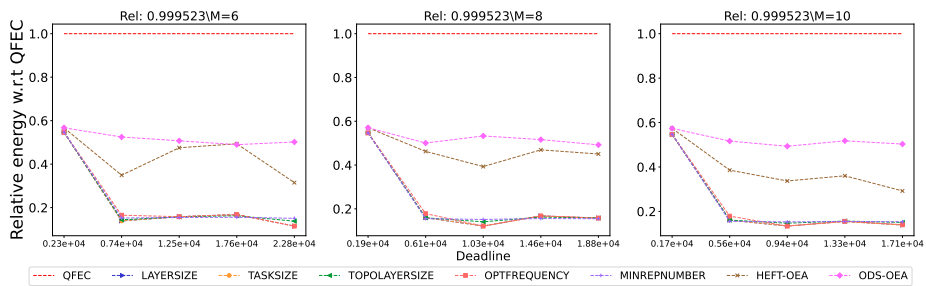
Figure 2980: Assessing the performance of different processor number on the BWA workflow.
