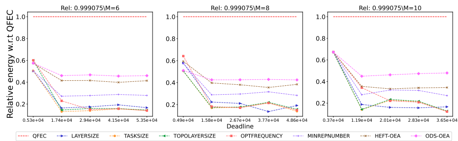
Figure 2807: Assessing the performance of different processor number on the Epigenomics workflow.
