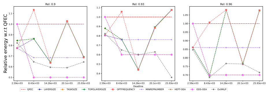
Figure 1480: Assessing the performance of EXTMILP on the SRASearch workflow (with 10 tasks).
