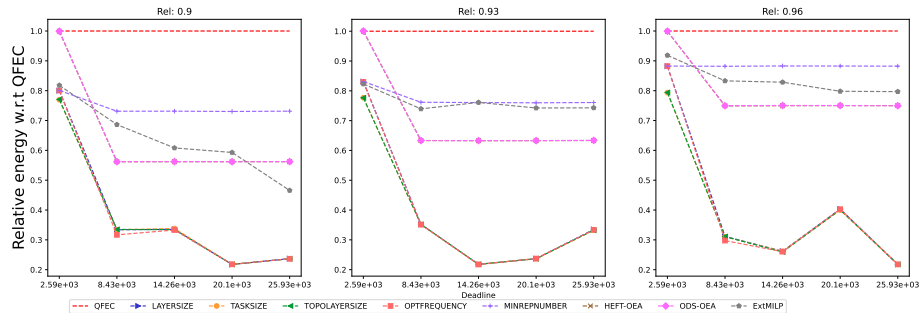
Figure 1280: Assessing the performance of EXTMLP on the SRASearch workflow (with 10 tasks).
