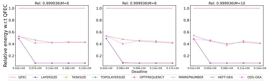
Figure 2867: Assessing the performance of different processor number on the Seismology workflow.
