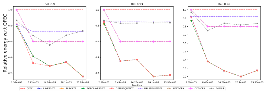
Figure 1140: Assessing the performance of EXTMLP on the SRASearch workflow (with 10 tasks).
