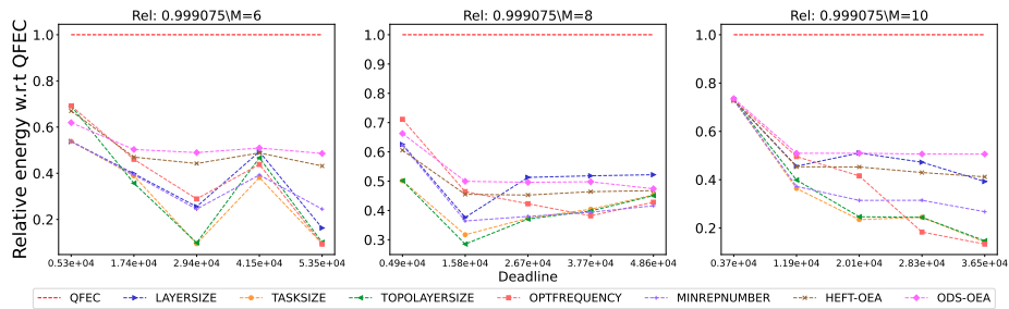
Figure 2565: Assessing the performance of different processor number on the Epigenomics workflow.
