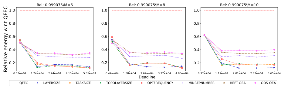
Figure 2664: Assessing the performance of different processor number on the Epigenomics workflow.
