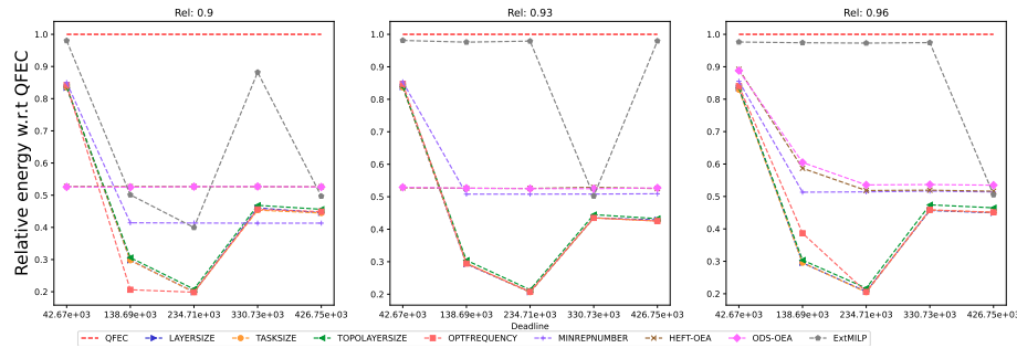
Figure 898: Assessing the performance of EXT MILP on the SoyKB workflow (with 20 tasks).
