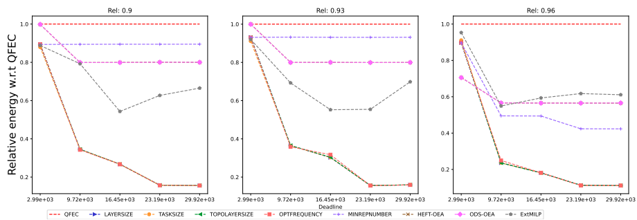
Figure 1061: Assessing the performance of EXTMILP on the SRASearch workflow (with 20 tasks).
