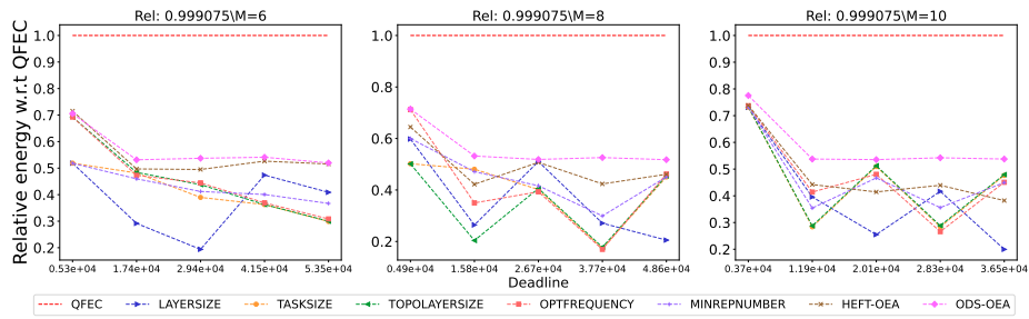
Figure 3016: Assessing the performance of different processor number on the Epigenomics workflow.
