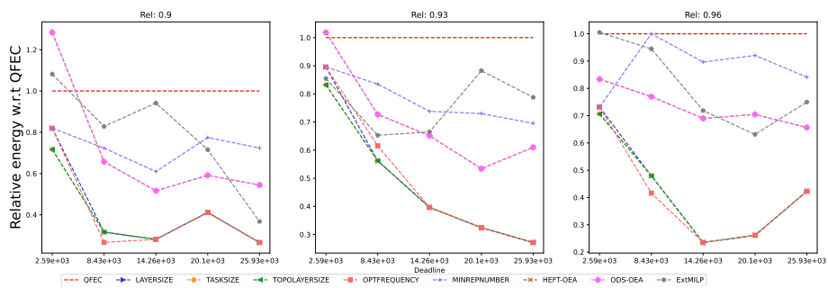
Figure 1580: Assessing the performance of EXTMLP on the SRASearch workflow (with 10 tasks).
