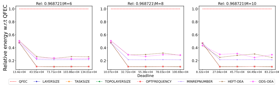
Figure 2715: Assessing the performance of different processor number on the BLAST workflow.
