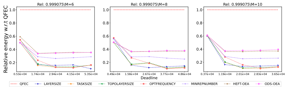
Figure 2642: Assessing the performance of different processor number on the Epigenomics workflow.
