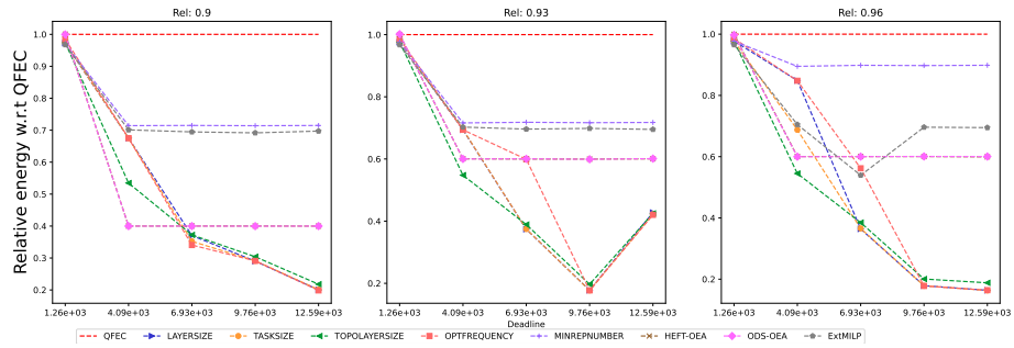
Figure 1130: Assessing the performance of EXTMILP on the Epigenomics workflow (with 20 tasks).
