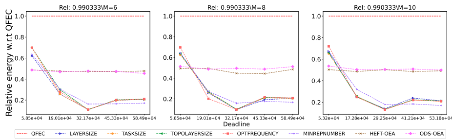
Figure 2912: Assessing the performance of different processor number on the SoyKB workflow.
