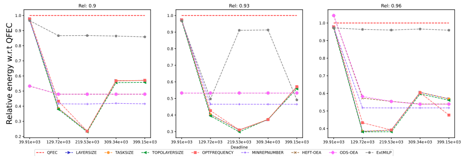
Figure 1479: Assessing the performance of EXTMILP on the SoyKB workflow (with 30 tasks).
