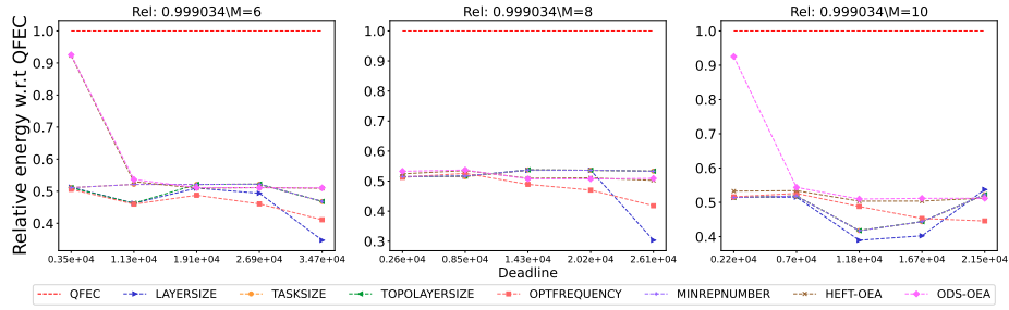
Figure 2607: Assessing the performance of different processor number on the Cholesky workflow.
