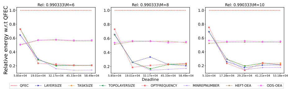
Figure 2989: Assessing the performance of different processor number on the SoyKB workflow.
