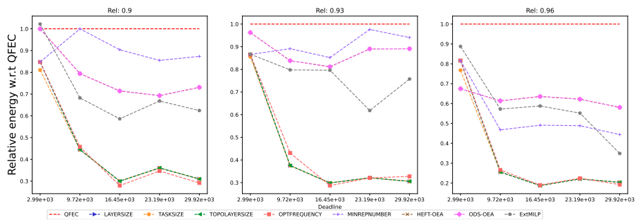
Figure 1581: Assessing the performance of EXTMLP on the SRASearch workflow (with 20 tasks).
