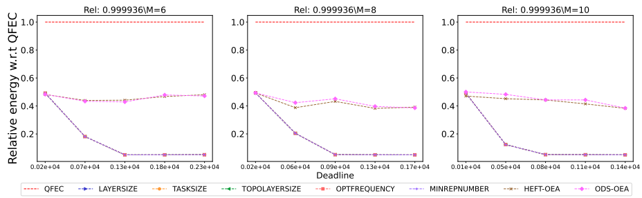
Figure 2482: Assessing the performance of different processor number on the Seismology workflow.
