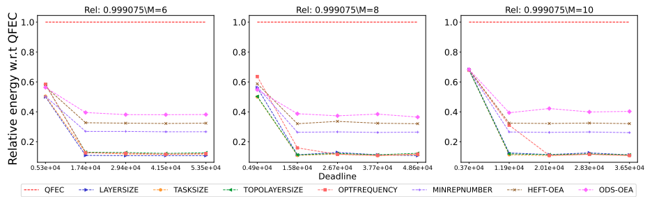
Figure 2323: Assessing the performance of different processor number on the Epigenomics workflow.
