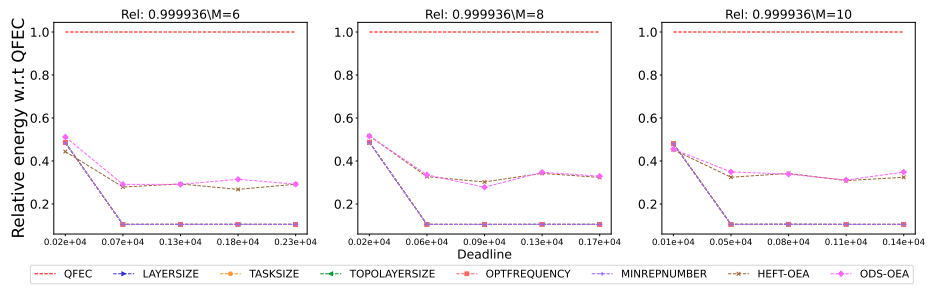
Figure 2317: Assessing the performance of different processor number on the Seismology workflow.
