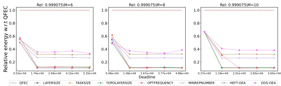
Figure 2279: Assessing the performance of different processor number on the Epigenomics workflow.
