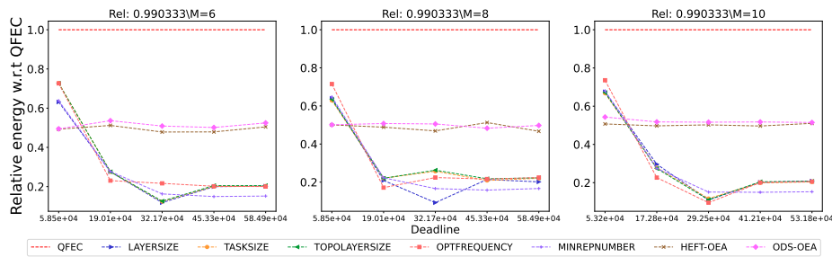
Figure 2538: Assessing the performance of different processor number on the SoyKB workflow.
