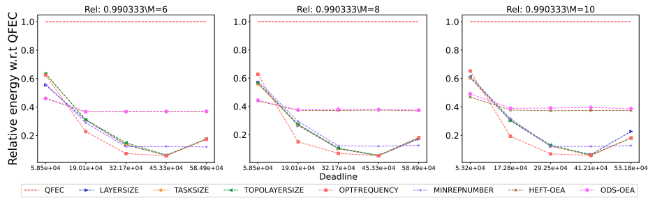
Figure 2351: Assessing the performance of different processor number on the SoyKB workflow.
