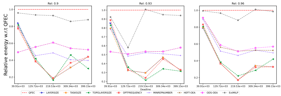
Figure 1839: Assessing the performance of EXTMILP on the SoyKB workflow (with 30 tasks).
