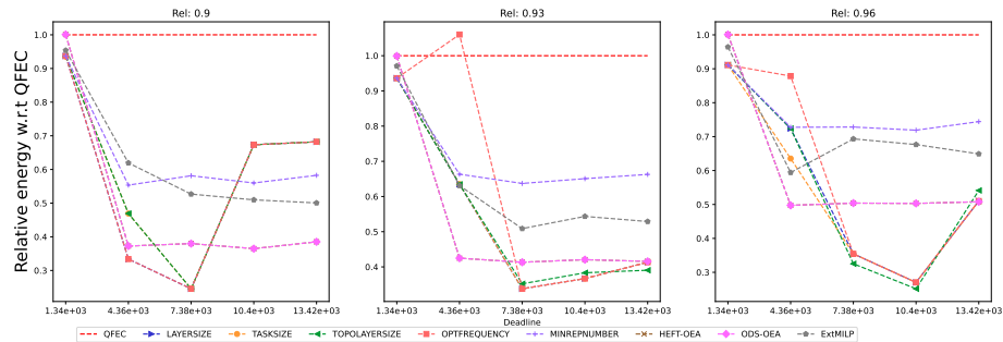
Figure 2063: Assessing the performance of EXT MILP on the BWA workflow (with 10 tasks).
