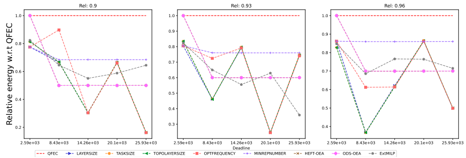
Figure 1320: Assessing the performance of EXTMILP on the SRASearch workflow (with 10 tasks).
