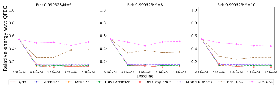
Figure 2892: Assessing the performance of different processor number on the BWA workflow.
