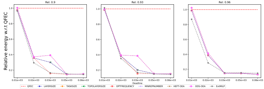
Figure 1536: Assessing the performance of EXTMILP on the Seismology workflow (with 20 tasks).
