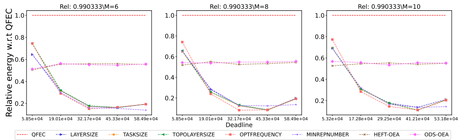
Figure 2571: Assessing the performance of different processor number on the SoyKB workflow.
