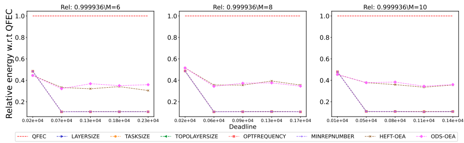
Figure 2757: Assessing the performance of different processor number on the Seismology workflow.
