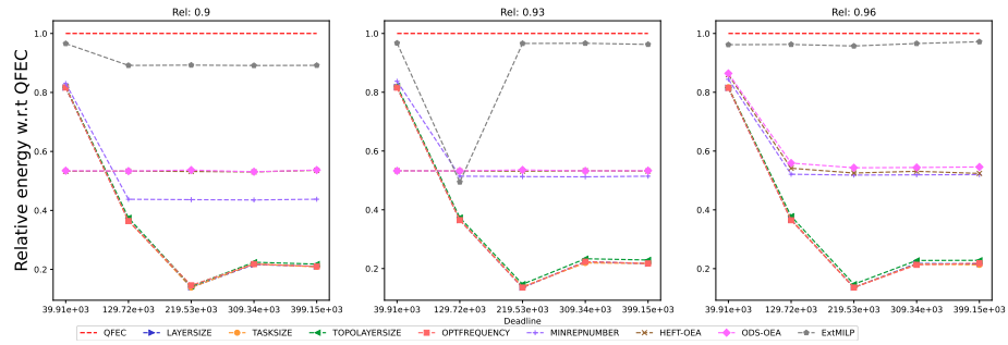
Figure 879: Assessing the performance of EXT MILP on the SoyKB workflow (with 30 tasks).
