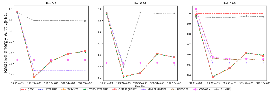
Figure 1519: Assessing the performance of EXTMLP on the SoyKB workflow (with 30 tasks).
