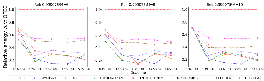
Figure 2906: Assessing the performance of different processor number on the Epigenomics workflow.
