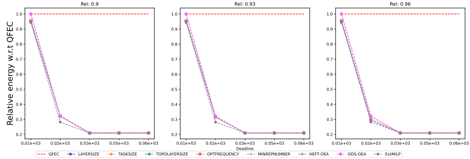
Figure 1416: Assessing the performance of EXTMILP on the Seismology workflow (with 20 tasks).
