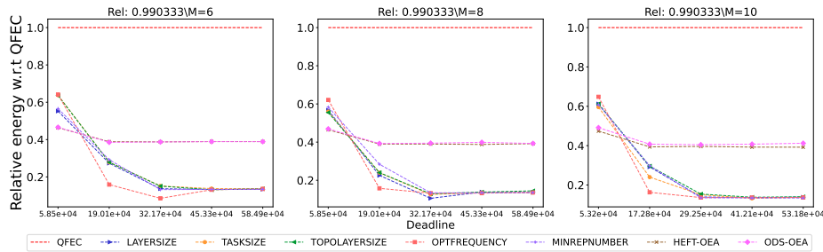
Figure 2373: Assessing the performance of different processor number on the SoyKB workflow.
