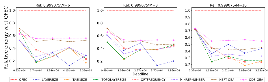
Figure 2950: Assessing the performance of different processor number on the Epigenomics workflow.
