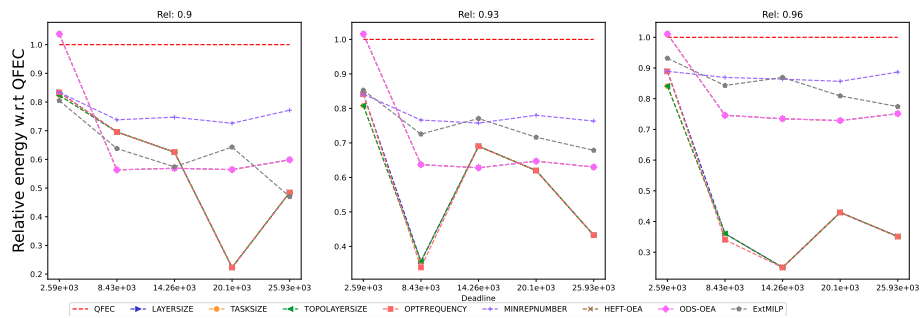
Figure 2080: Assessing the performance of EXTMLP on the SRASearch workflow (with 10 tasks).
