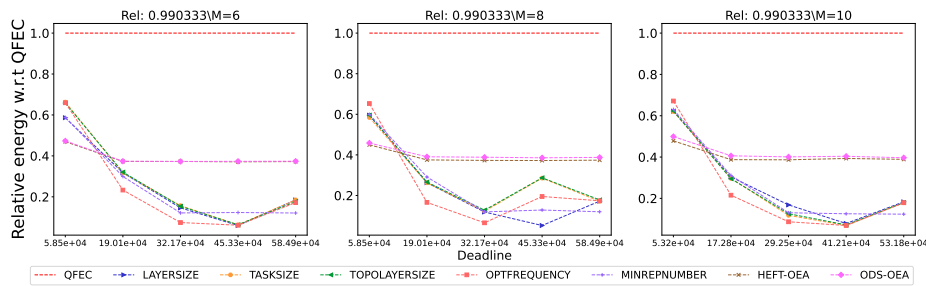
Figure 2395: Assessing the performance of different processor number on the SoyKB workflow.
