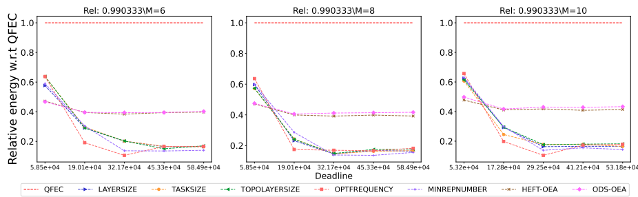
Figure 2857: Assessing the performance of different processor number on the SoyKB workflow.
