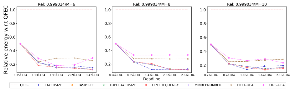
Figure 2662: Assessing the performance of different processor number on the Cholesky workflow.
