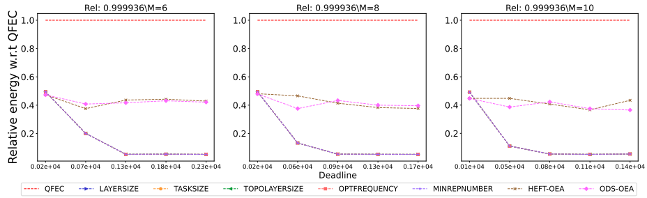
Figure 2834: Assessing the performance of different processor number on the Seismology workflow.
