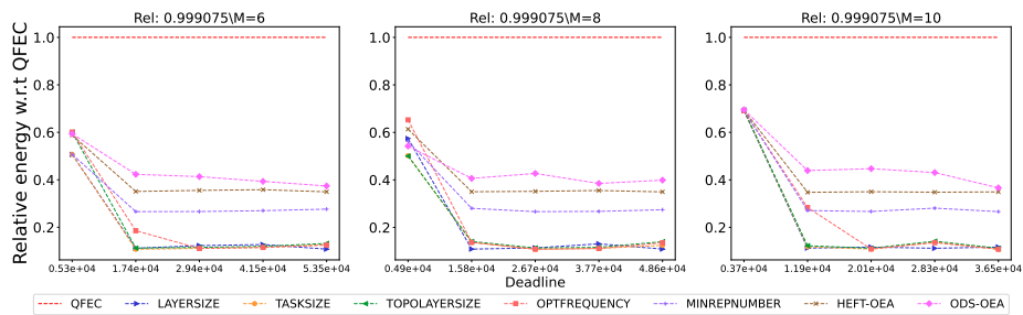
Figure 2356: Assessing the performance of different processor number on the Epigenomics workflow.
