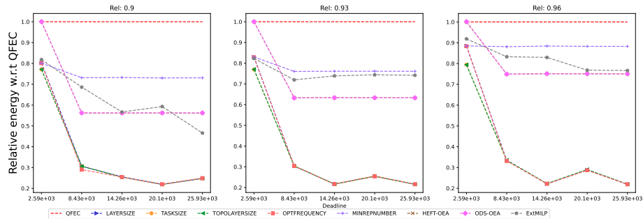
Figure 1120: Assessing the performance of EXTMLP on the SRASearch workflow (with 10 tasks).
