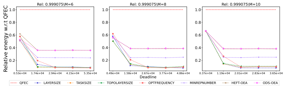
Figure 2246: Assessing the performance of different processor number on the Epigenomics workflow.
