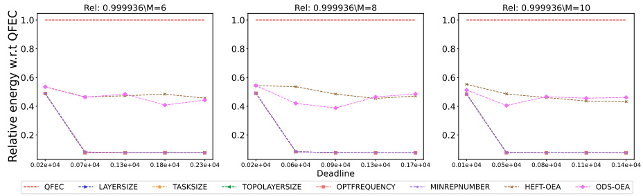
Figure 2911: Assessing the performance of different processor number on the Seismology workflow.
