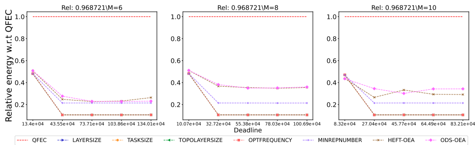
Figure 2363: Assessing the performance of different processor number on the BLAST workflow.
