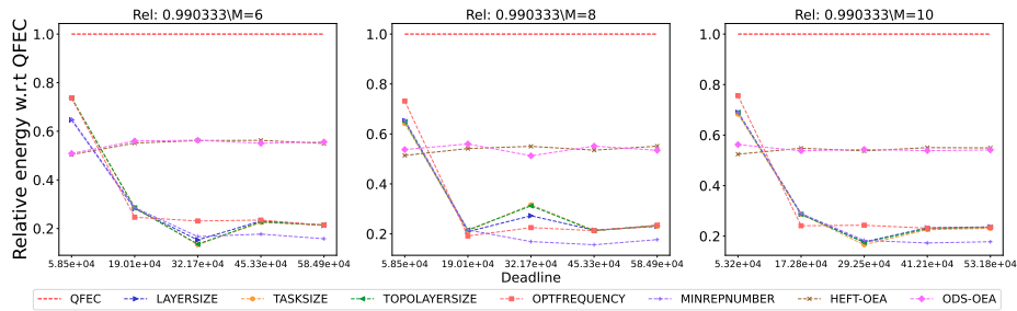
Figure 2978: Assessing the performance of different processor number on the SoyKB workflow.
