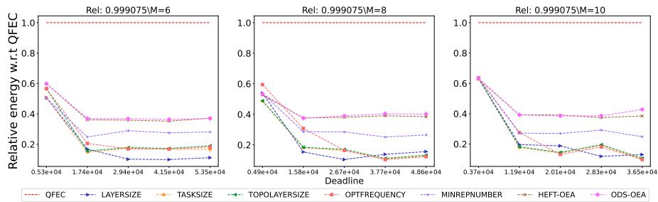
Figure 2686: Assessing the performance of different processor number on the Epigenomics workflow.
