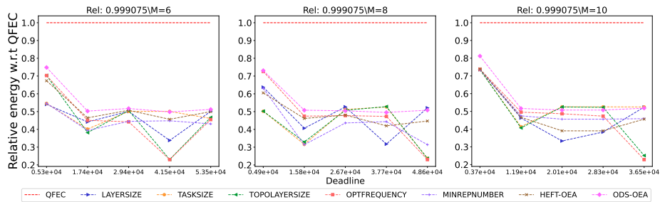
Figure 2609: Assessing the performance of different processor number on the Epigenomics workflow.
