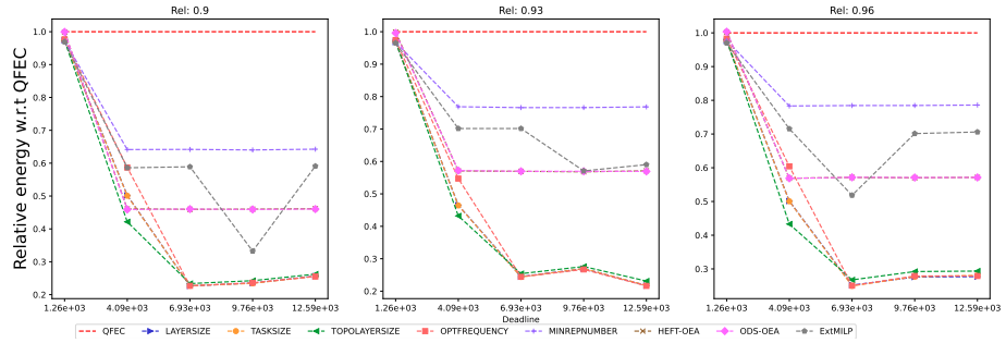
Figure 1010: Assessing the performance of EXTMILP on the Epigenomics workflow (with 20 tasks).
