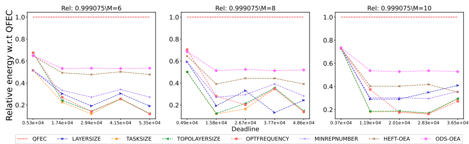
Figure 2576: Assessing the performance of different processor number on the Epigenomics workflow.
