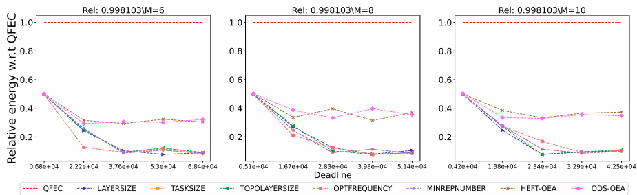
Figure 2338: Assessing the performance of different processor number on the QR.
