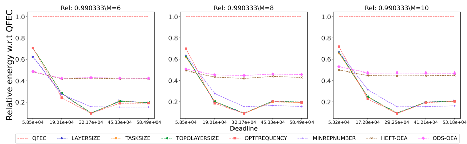
Figure 2472: Assessing the performance of different processor number on the SoyKB workflow.
