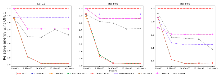
Figure 861: Assessing the performance of EXTMLP on the SRASearch workflow (with 20 tasks).
