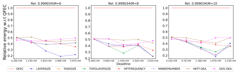
Figure 2915: Assessing the performance of different processor number on the Cholesky workflow.
