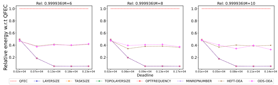
Figure 2790: Assessing the performance of different processor number on the Seismology workflow.
