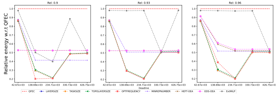
Figure 978: Assessing the performance of EXTMLP on the SoyKB workflow (with 20 tasks).
