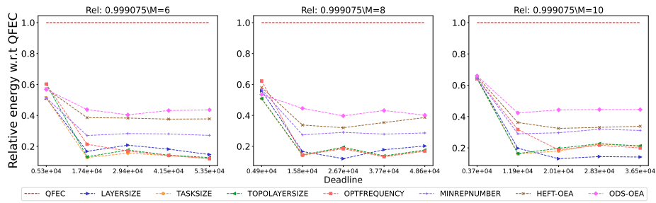
Figure 2763: Assessing the performance of different processor number on the Epigenomics workflow.
