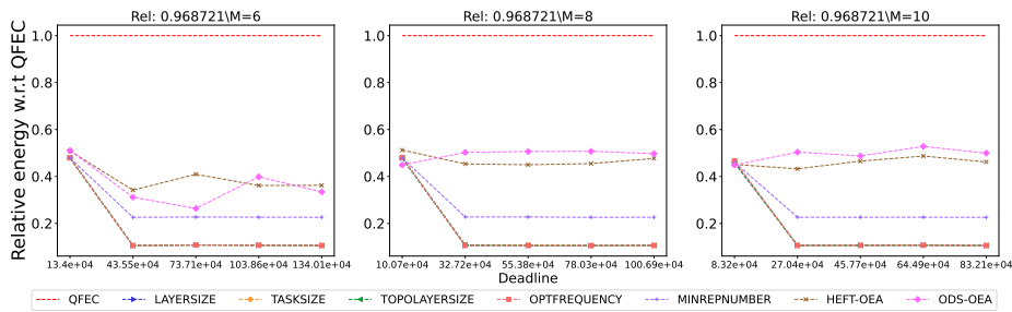
Figure 2836: Assessing the performance of different processor number on the BLAST workflow.
