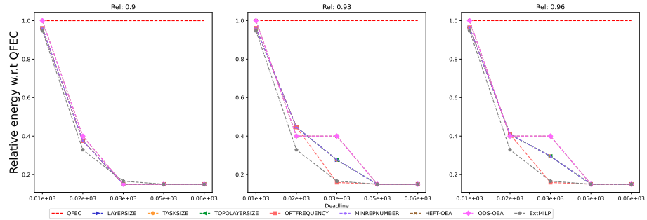
Figure 1376: Assessing the performance of EXTMILP on the Seismology workflow (with 20 tasks).
