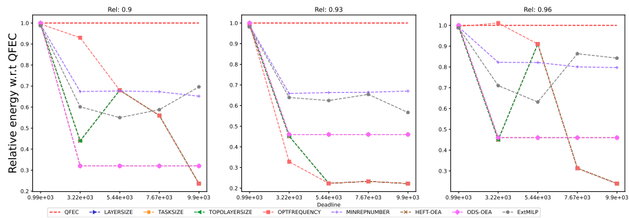
Figure 1889: Assessing the performance of EXTMLP on the Epigenomics workflow (with 10 tasks).
