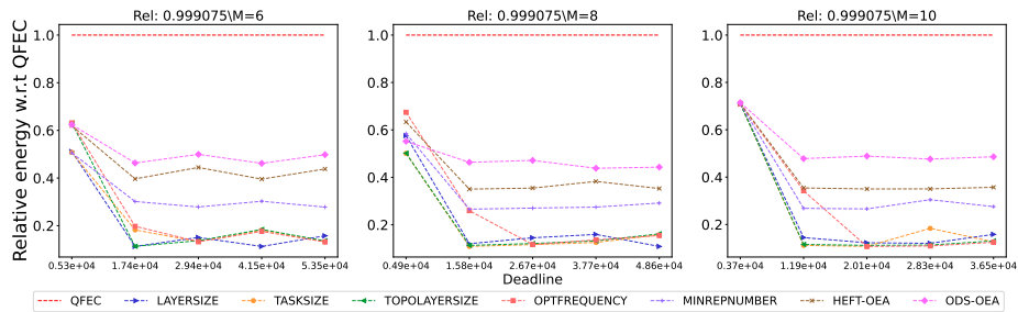
Figure 2444: Assessing the performance of different processor number on the Epigenomics workflow.
