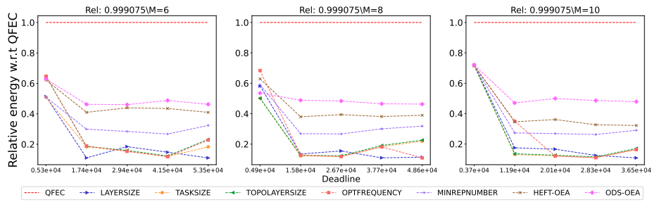
Figure 2499: Assessing the performance of different processor number on the Epigenomics workflow.
