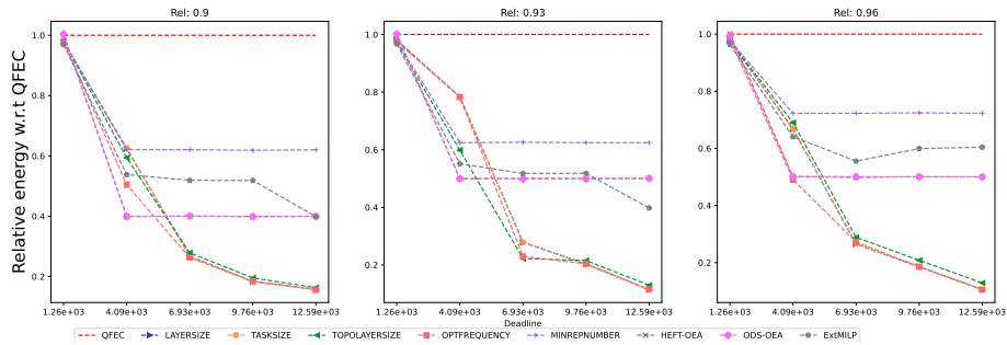
Figure 830: Assessing the performance of EXTMLP on the Epigenomics workflow (with 20 tasks).
