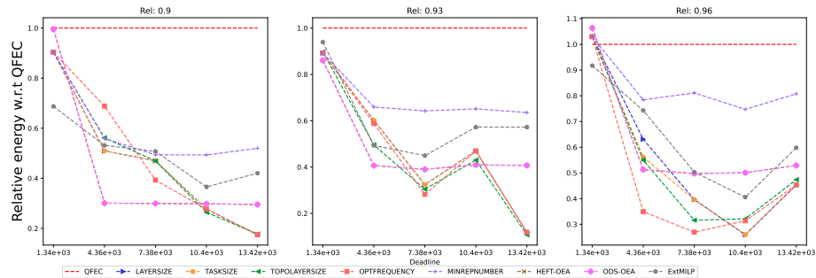
Figure 1623: Assessing the performance of EXT MILP on the BWA workflow (with 10 tasks).
