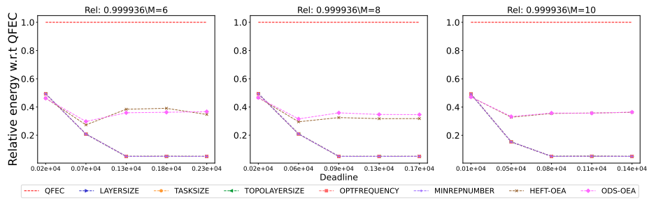
Figure 2306: Assessing the performance of different processor number on the Seismology workflow.
