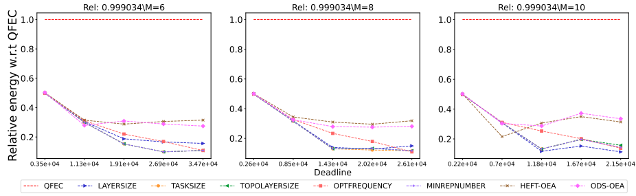
Figure 2684: Assessing the performance of different processor number on the Cholesky workflow.
