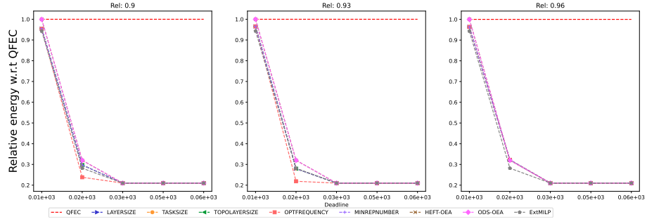
Figure 1256: Assessing the performance of EXTMILP on the Seismology workflow (with 20 tasks).
