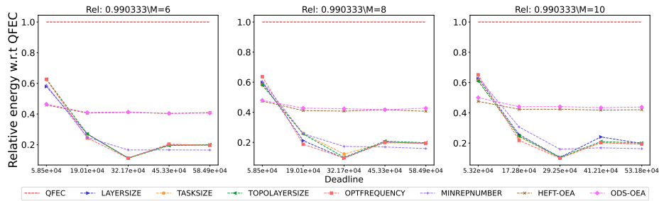
Figure 2824: Assessing the performance of different processor number on the SoyKB workflow.
