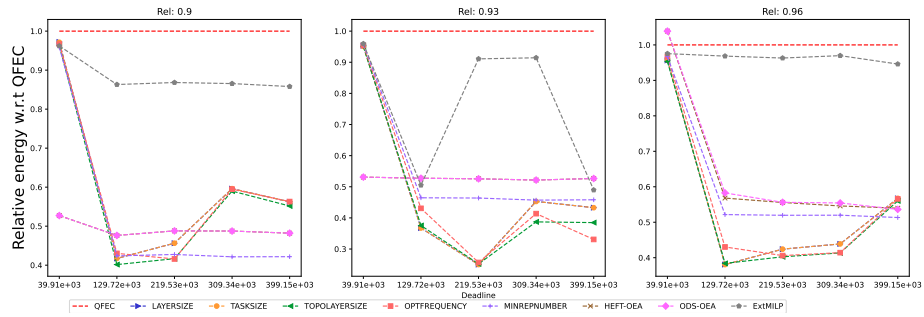
Figure 2199: Assessing the performance of EXTMILP on the SoyKB workflow (with 30 tasks).
