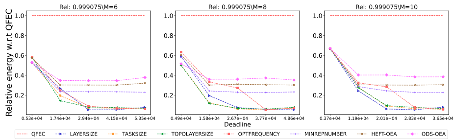
Figure 2257: Assessing the performance of different processor number on the Epigenomics workflow.
