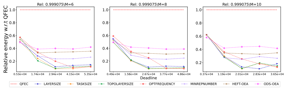
Figure 2697: Assessing the performance of different processor number on the Epigenomics workflow.
