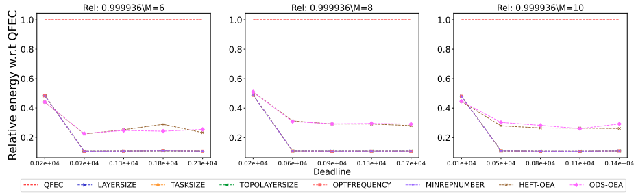
Figure 2669: Assessing the performance of different processor number on the Seismology workflow.
