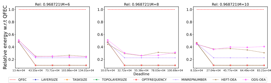
Figure 2352: Assessing the performance of different processor number on the BLAST workflow.
