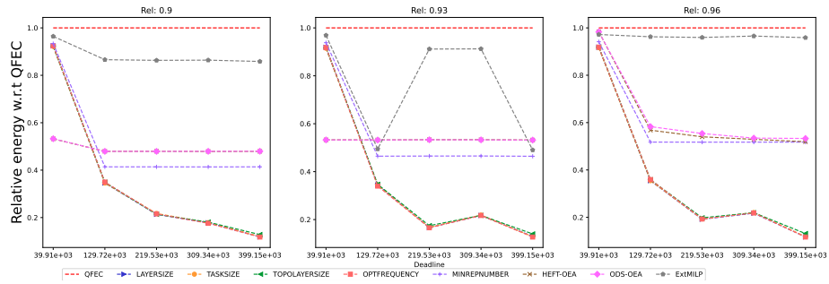
Figure 1239: Assessing the performance of EXTMILP on the SoyKB workflow (with 30 tasks).
