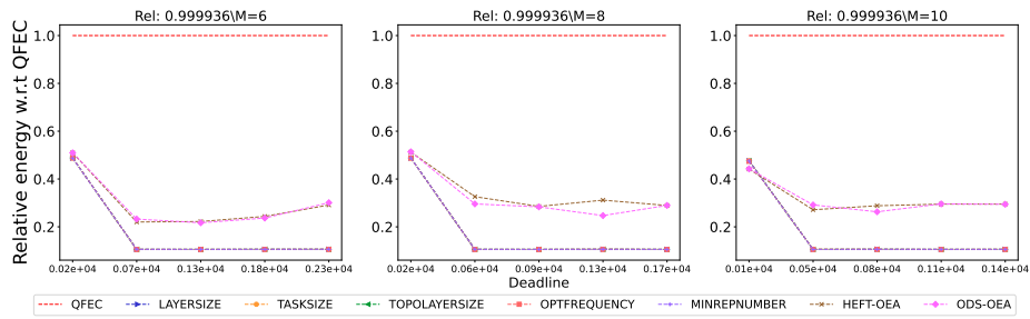
Figure 2284: Assessing the performance of different processor number on the Seismology workflow.
