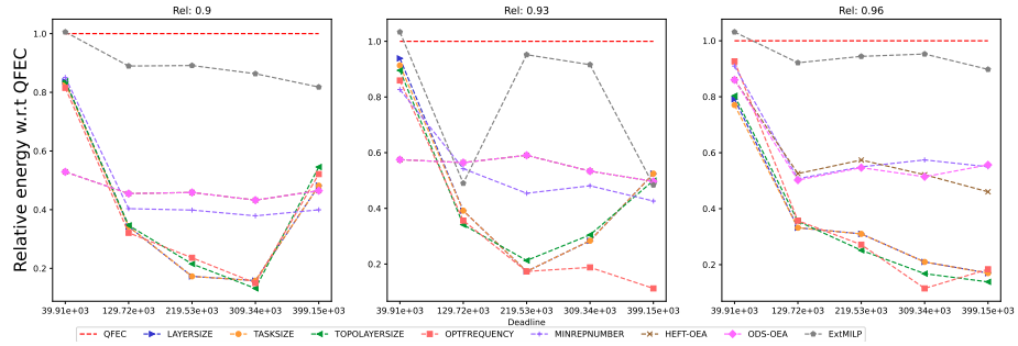
Figure 1799: Assessing the performance of EXTMILP on the SoyKB workflow (with 30 tasks).
