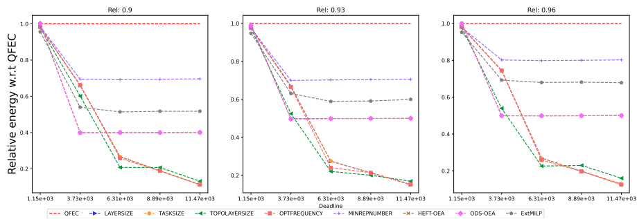
Figure 831: Assessing the performance of EXTMLP on the Epigenomics workflow (with 30 tasks).
