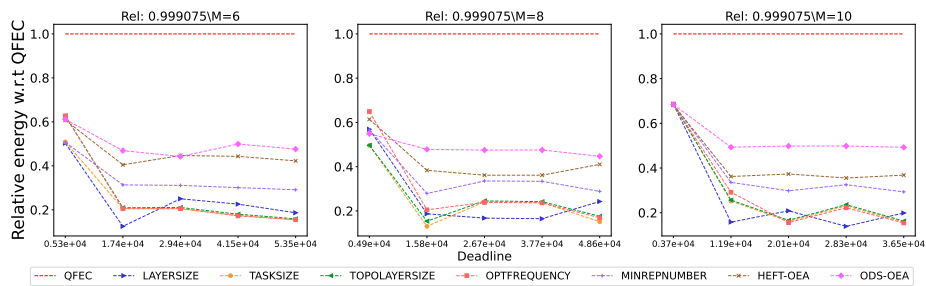
Figure 2840: Assessing the performance of different processor number on the Epigenomics workflow.
