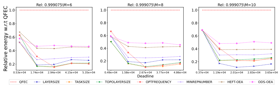
Figure 2818: Assessing the performance of different processor number on the Epigenomics workflow.
