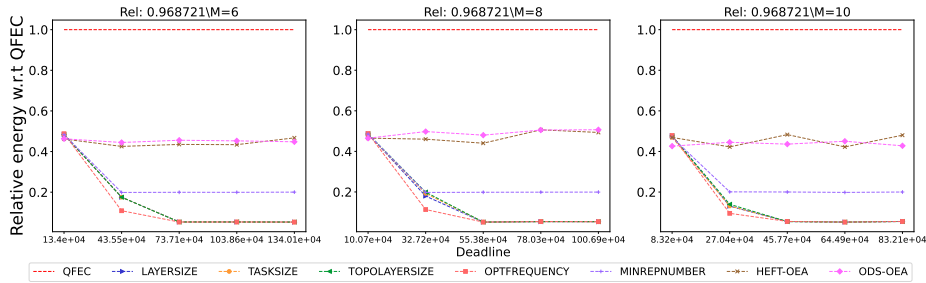
Figure 2825: Assessing the performance of different processor number on the BLAST workflow.
