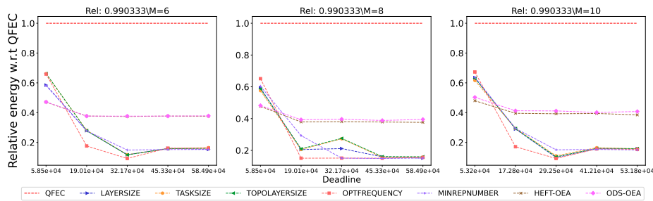
Figure 2406: Assessing the performance of different processor number on the SoyKB workflow.
