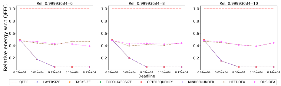
Figure 2878: Assessing the performance of different processor number on the Seismology workflow.
