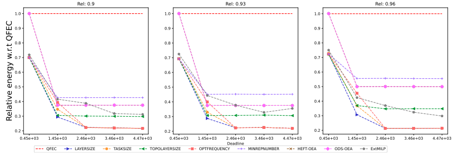
Figure 1033: Assessing the performance of EXT MILP on the Genome workflow (with 20 tasks).
