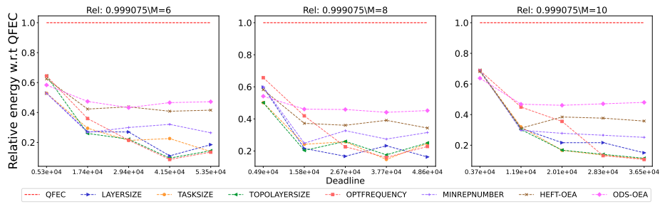
Figure 2829: Assessing the performance of different processor number on the Epigenomics workflow.
