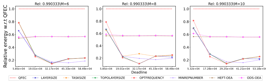
Figure 3022: Assessing the performance of different processor number on the SoyKB workflow.
