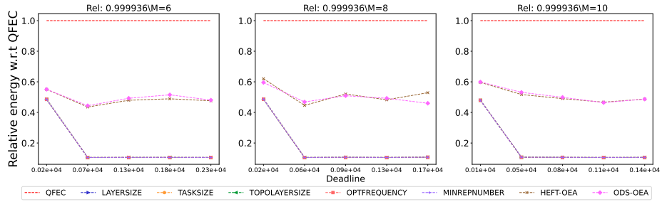
Figure 2977: Assessing the performance of different processor number on the Seismology workflow.
