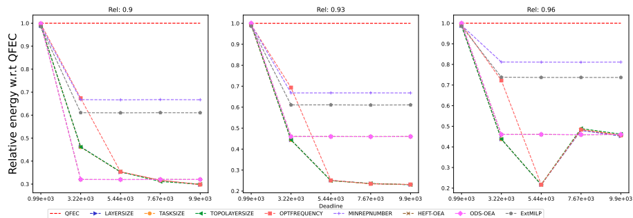
Figure 1249: Assessing the performance of EXTMLP on the Epigenomics workflow (with 10 tasks).
