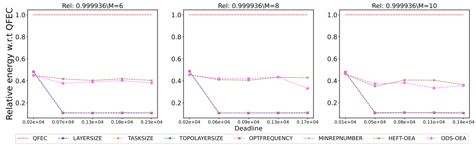
Figure 2801: Assessing the performance of different processor number on the Seismology workflow.
