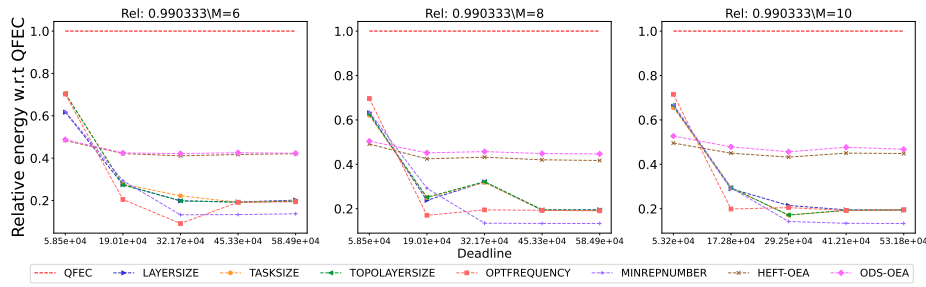
Figure 2505: Assessing the performance of different processor number on the SoyKB workflow.
