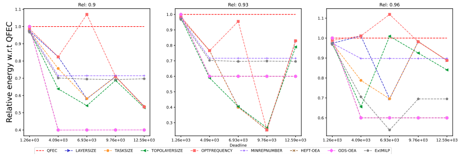
Figure 1370: Assessing the performance of EXTMILP on the Epigenomics workflow (with 20 tasks).
