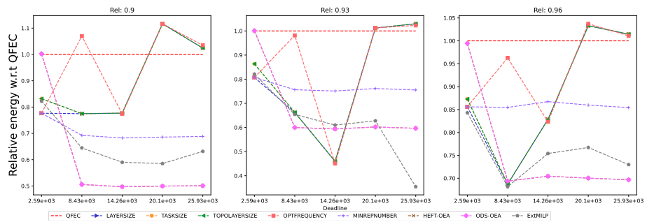
Figure 2200: Assessing the performance of EXTMILP on the SRASearch workflow (with 10 tasks).
