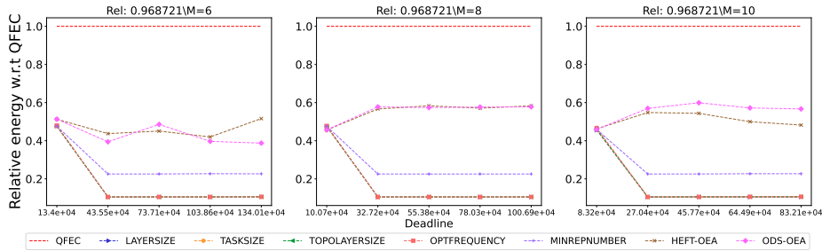
Figure 2484: Assessing the performance of different processor number on the BLAST workflow.
