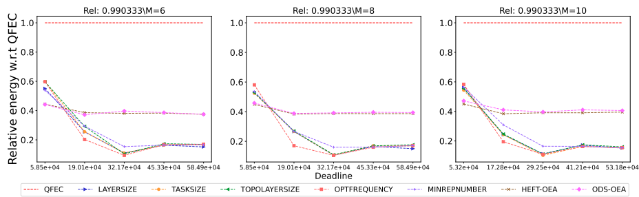
Figure 2736: Assessing the performance of different processor number on the SoyKB workflow.
