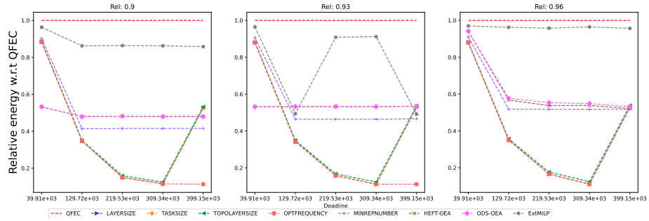
Figure 1079: Assessing the performance of EXTMLP on the SoyKB workflow (with 30 tasks).
