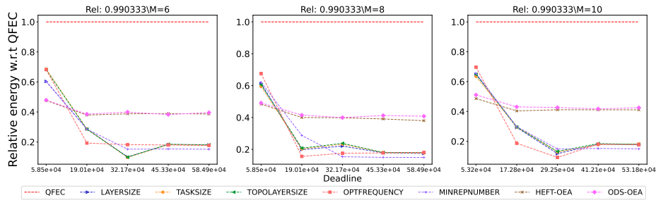
Figure 2450: Assessing the performance of different processor number on the SoyKB workflow.
