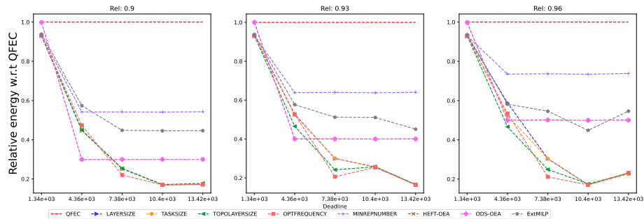
Figure 983: Assessing the performance of EXTMILP on the BWA workflow (with 10 tasks).
