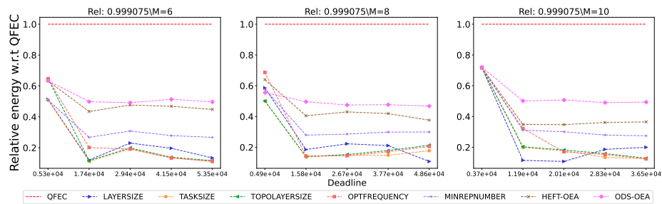
Figure 2488: Assessing the performance of different processor number on the Epigenomics workflow.
