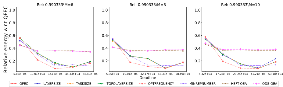
Figure 2747: Assessing the performance of different processor number on the SoyKB workflow.
