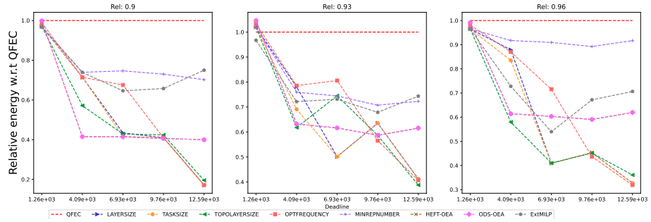
Figure 1850: Assessing the performance of EXTMILP on the Epigenomics workflow (with 20 tasks).
