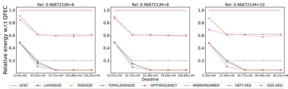
Figure 3001: Assessing the performance of different processor number on the BLAST workflow.
