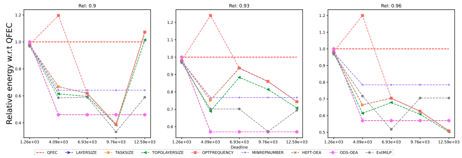
Figure 1490: Assessing the performance of EXTMILP on the Epigenomics workflow (with 20 tasks).
