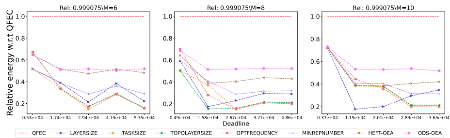
Figure 2972: Assessing the performance of different processor number on the Epigenomics workflow.
