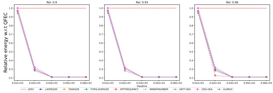
Figure 1016: Assessing the performance of EXTMILP on the Seismology workflow (with 20 tasks).
