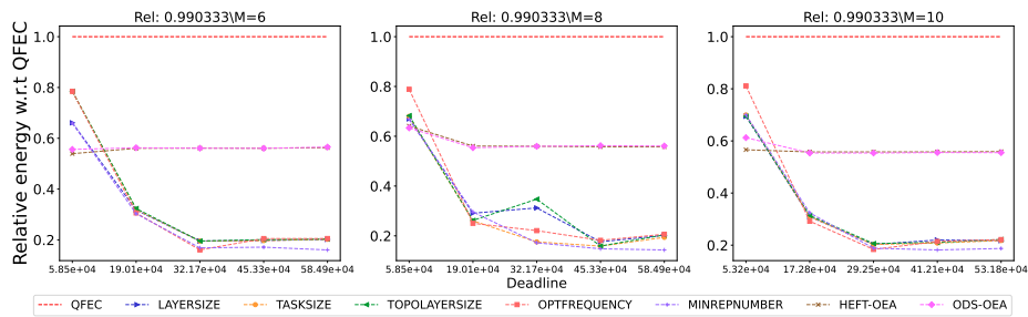
Figure 3011: Assessing the performance of different processor number on the SoyKB workflow.
