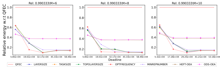
Figure 2362: Assessing the performance of different processor number on the SoyKB workflow.
