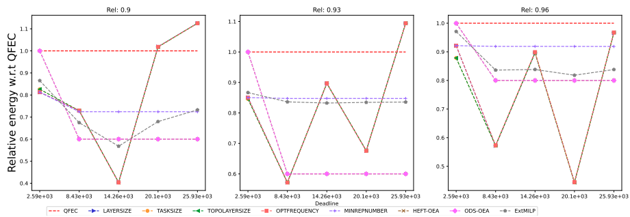
Figure 1460: Assessing the performance of EXTMLP on the SRASearch workflow (with 10 tasks).
