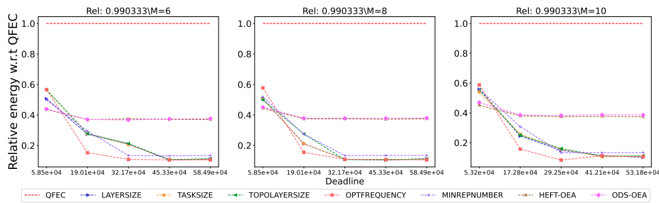
Figure 2285: Assessing the performance of different processor number on the SoyKB workflow.
