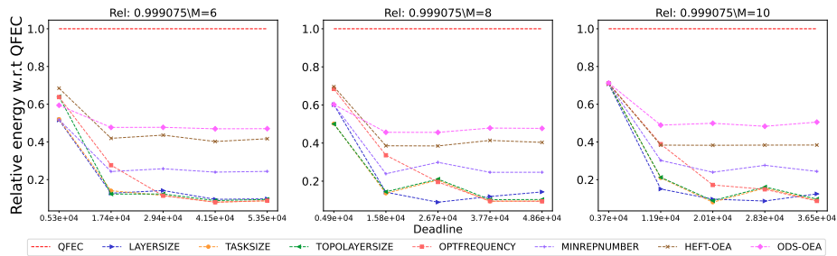
Figure 2422: Assessing the performance of different processor number on the Epigenomics workflow.
