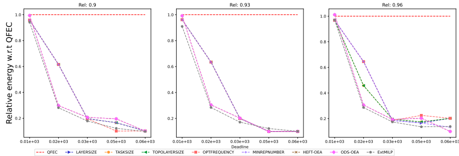
Figure 1876: Assessing the performance of EXT MILP on the Seismology workflow (with 20 tasks).
