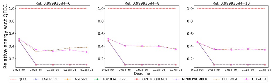
Figure 2361: Assessing the performance of different processor number on the Seismology workflow.
