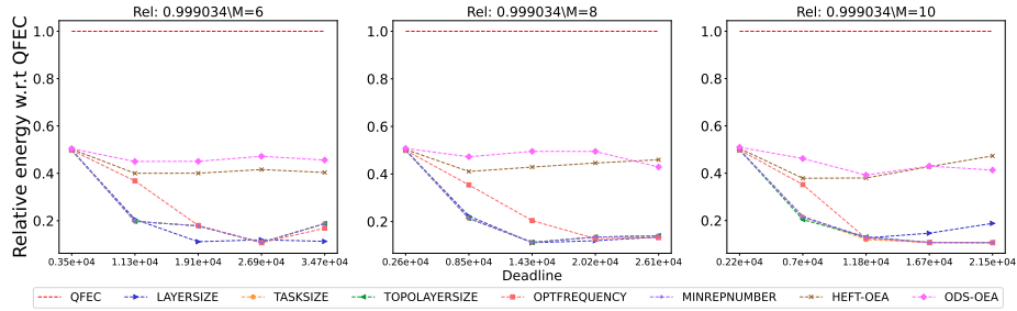
Figure 2442: Assessing the performance of different processor number on the Cholesky workflow.
