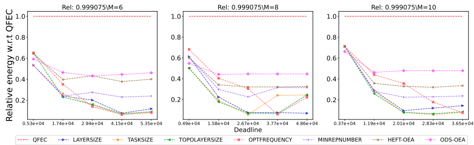
Figure 2433: Assessing the performance of different processor number on the Epigenomics workflow.
