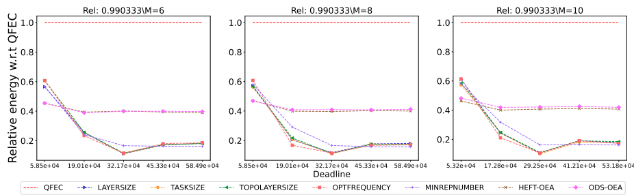
Figure 2780: Assessing the performance of different processor number on the SoyKB workflow.
