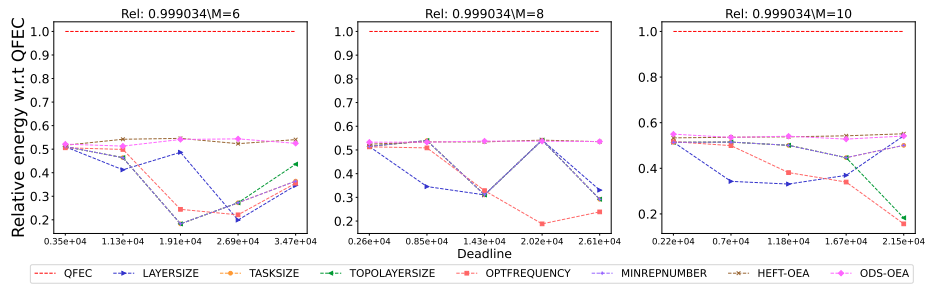
Figure 3025: Assessing the performance of different processor number on the Cholesky workflow.
