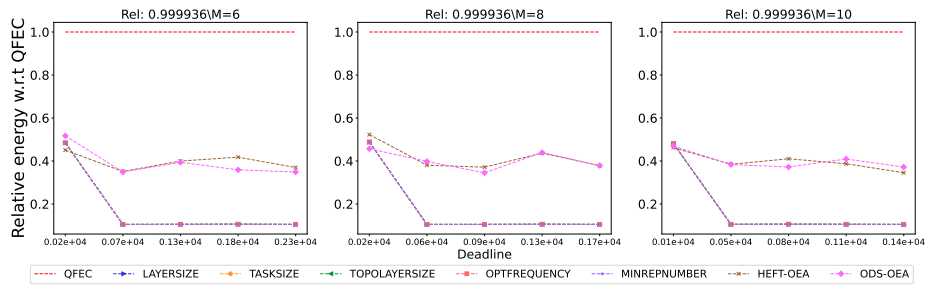
Figure 2405: Assessing the performance of different processor number on the Seismology workflow.
