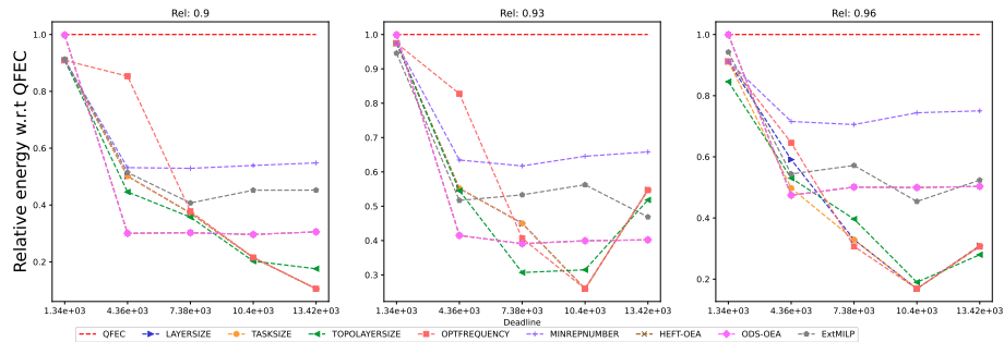
Figure 1863: Assessing the performance of EXT MILP on the BWA workflow (with 10 tasks).
