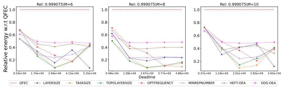
Figure 2521: Assessing the performance of different processor number on the Epigenomics workflow.
