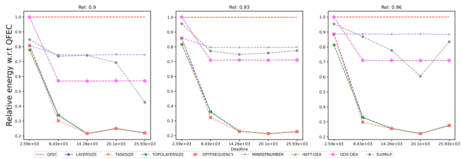
Figure 1020: Assessing the performance of EXTMLP on the SRASearch workflow (with 10 tasks).
