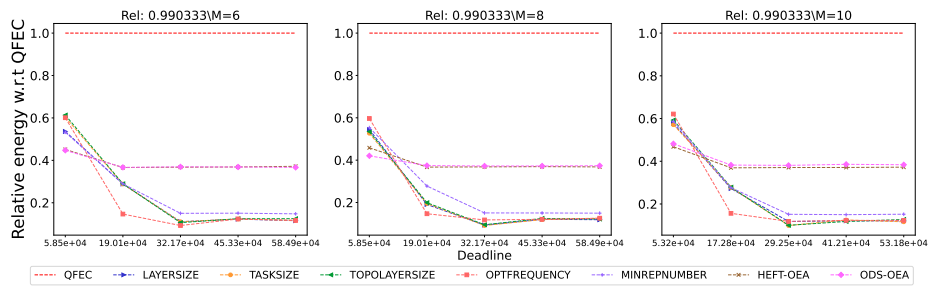
Figure 2318: Assessing the performance of different processor number on the SoyKB workflow.
