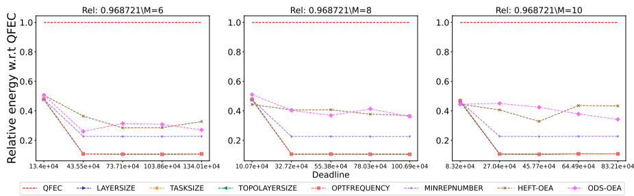
Figure 2792: Assessing the performance of different processor number on the BLAST workflow.
