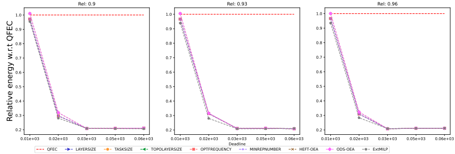
Figure 2136: Assessing the performance of EXTMILP on the Seismology workflow (with 20 tasks).
