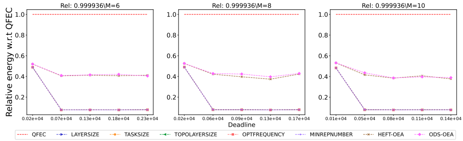
Figure 2823: Assessing the performance of different processor number on the Seismology workflow.
