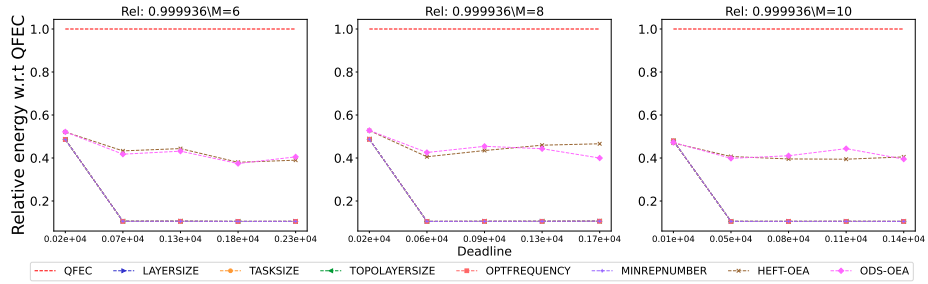
Figure 2449: Assessing the performance of different processor number on the Seismology workflow.
