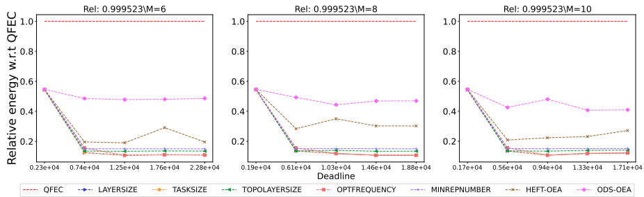
Figure 2452: Assessing the performance of different processor number on the BWA workflow.
