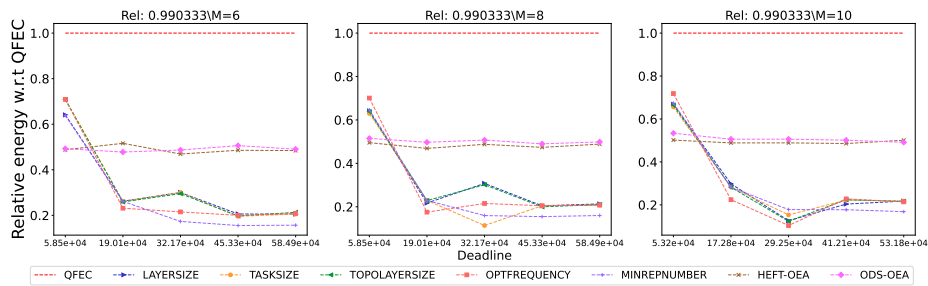
Figure 2934: Assessing the performance of different processor number on the SoyKB workflow.
