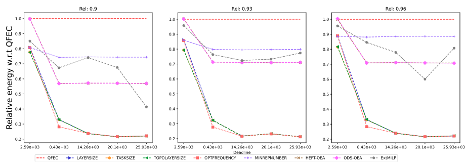
Figure 860: Assessing the performance of EXTMLP on the SRASearch workflow (with 10 tasks).
