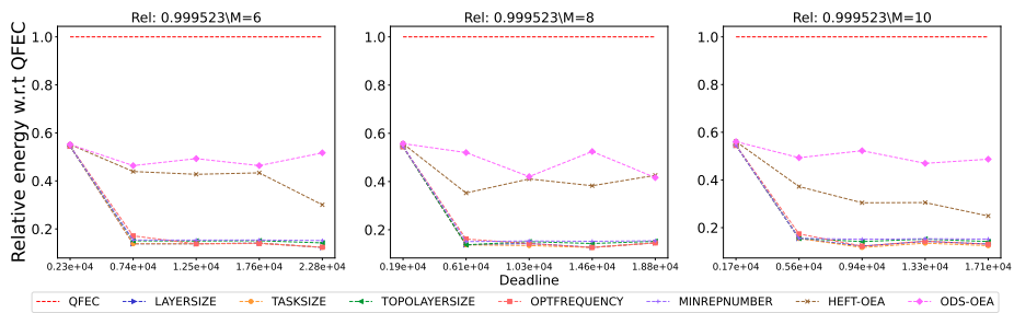
Figure 2936: Assessing the performance of different processor number on the BWA workflow.
