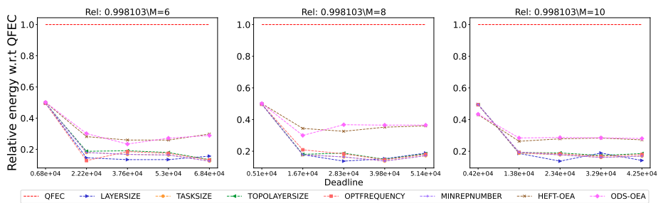
Figure 2712: Assessing the performance of different processor number on the QR.
