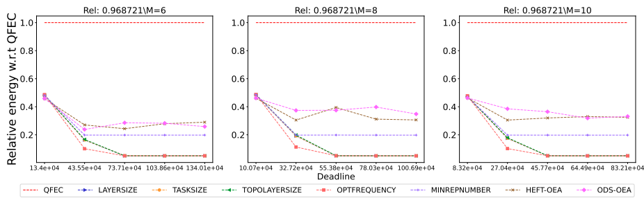
Figure 2341: Assessing the performance of different processor number on the BLAST workflow.
