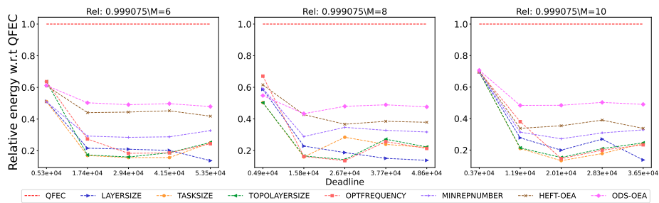
Figure 2895: Assessing the performance of different processor number on the Epigenomics workflow.
