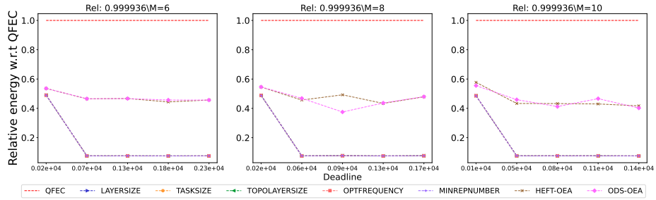
Figure 2515: Assessing the performance of different processor number on the Seismology workflow.
