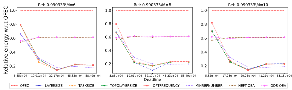
Figure 2604: Assessing the performance of different processor number on the SoyKB workflow.
