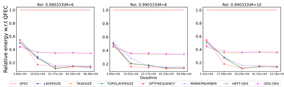
Figure 2714: Assessing the performance of different processor number on the SoyKB workflow.
