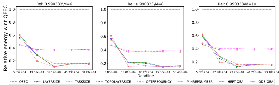
Figure 2802: Assessing the performance of different processor number on the SoyKB workflow.
