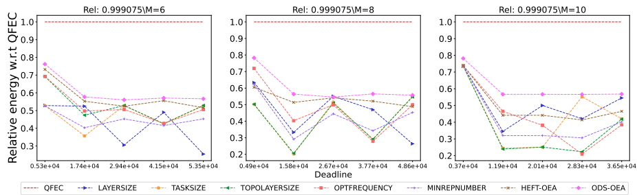
Figure 2598: Assessing the performance of different processor number on the Epigenomics workflow.
