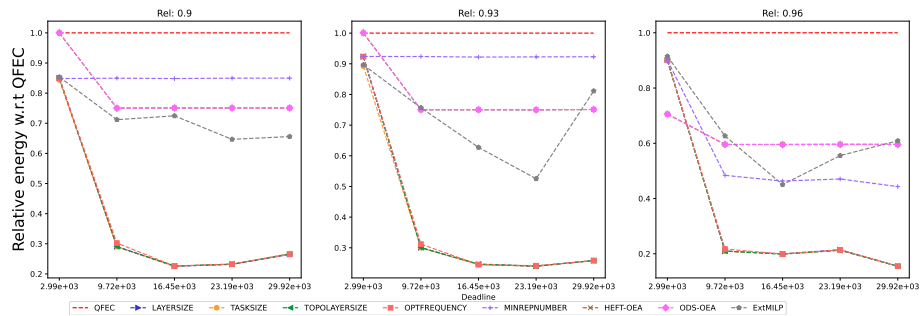
Figure 1121: Assessing the performance of EXTMLP on the SRASearch workflow (with 20 tasks).
