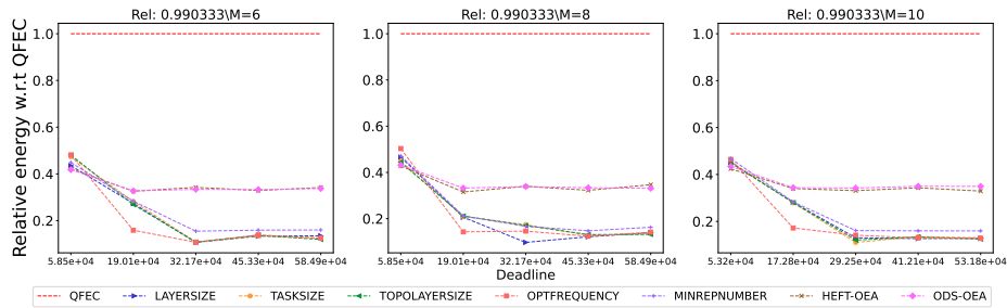
Figure 2670: Assessing the performance of different processor number on the SoyKB workflow.
