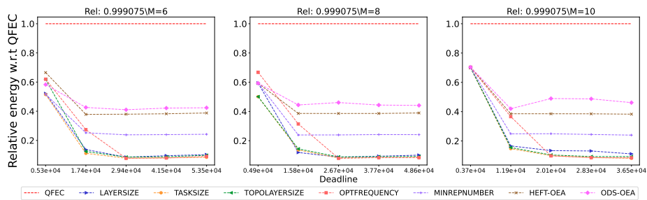
Figure 2378: Assessing the performance of different processor number on the Epigenomics workflow.
