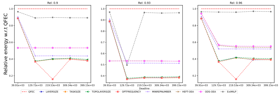
Figure 1119: Assessing the performance of EXTMLP on the SoyKB workflow (with 30 tasks).
