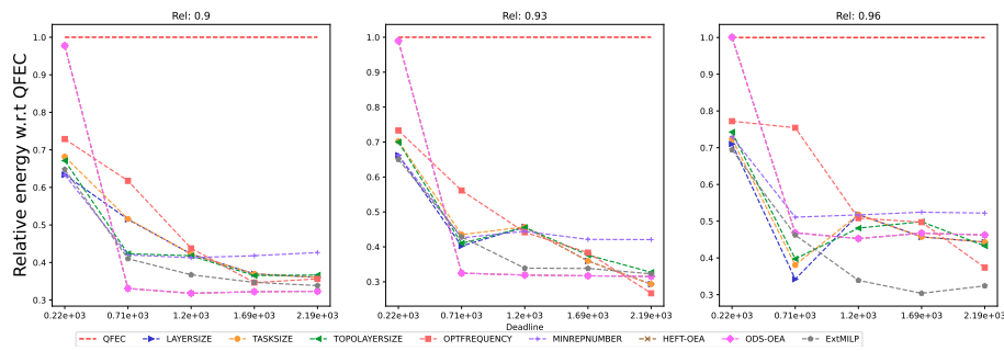
Figure 1888: Assessing the performance of EXTMLP on the Cycles workflow (with 30 tasks).
