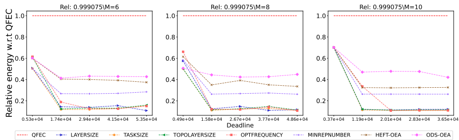
Figure 2411: Assessing the performance of different processor number on the Epigenomics workflow.
