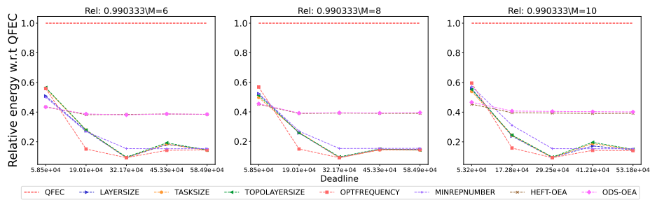
Figure 2252: Assessing the performance of different processor number on the SoyKB workflow.
