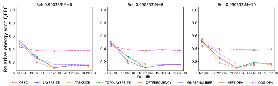
Figure 2692: Assessing the performance of different processor number on the SoyKB workflow.
