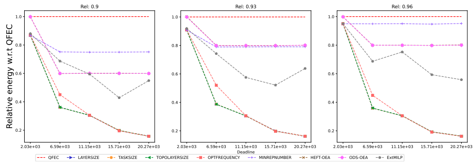
Figure 882: Assessing the performance of EXTMLP on the BLAST workflow (with 10 tasks).
