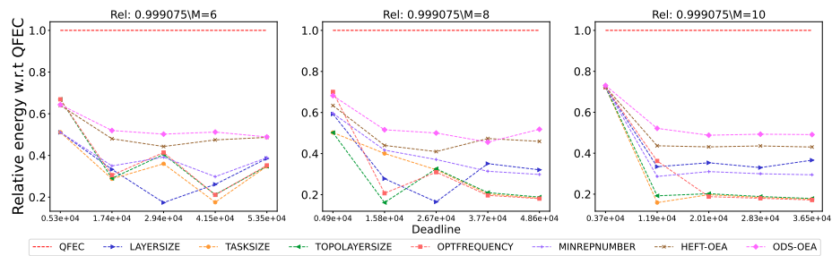
Figure 2983: Assessing the performance of different processor number on the Epigenomics workflow.
