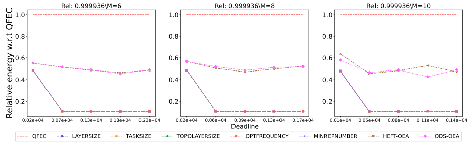
Figure 2592: Assessing the performance of different processor number on the Seismology workflow.
