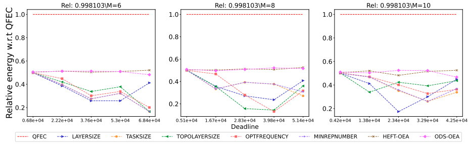
Figure 2954: Assessing the performance of different processor number on the QR.
