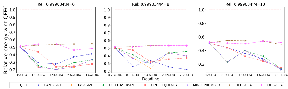
Figure 2574: Assessing the performance of different processor number on the Cholesky workflow.
