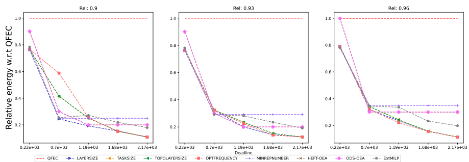
Figure 832: Assessing the performance of EXTMLP on the Genome workflow (with 10 tasks).
