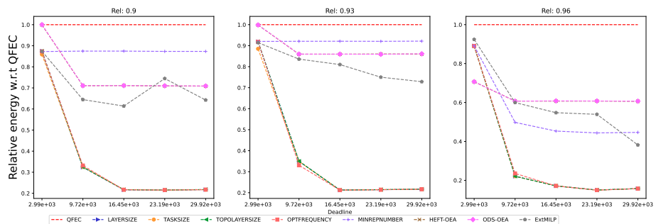
Figure 1021: Assessing the performance of EXTMLP on the SRASearch workflow (with 20 tasks).
