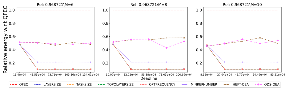
Figure 2495: Assessing the performance of different processor number on the BLAST workflow.
