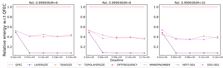
Figure 2427: Assessing the performance of different processor number on the Seismology workflow.
