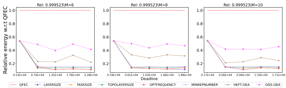
Figure 2848: Assessing the performance of different processor number on the BWA workflow.
