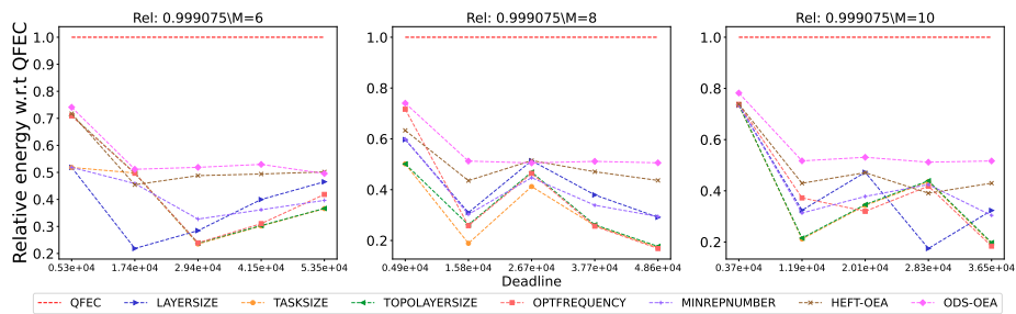
Figure 2631: Assessing the performance of different processor number on the Epigenomics workflow.
