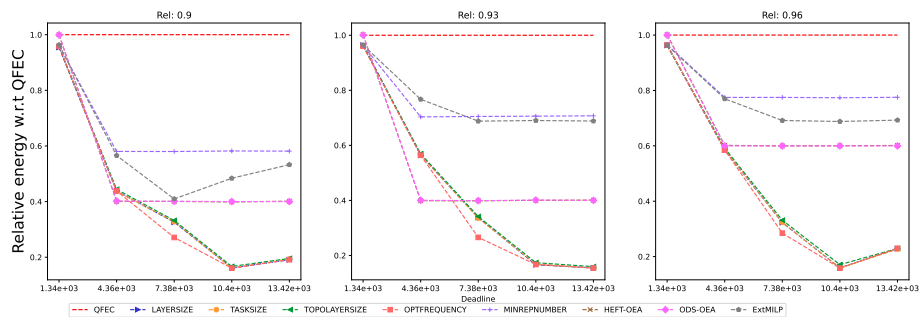
Figure 883: Assessing the performance of EXTMLP on the BWA workflow (with 10 tasks).
