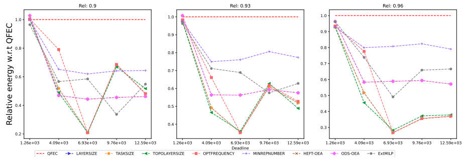
Figure 1890: Assessing the performance of EXTMILP on the Epigenomics workflow (with 20 tasks).
