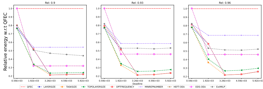
Figure 1007: Assessing the performance of EXT MILP on the Cycles workflow (with 20 tasks).
