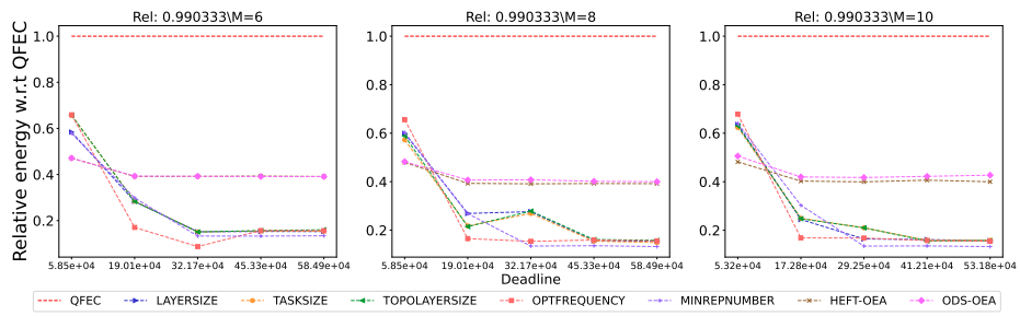
Figure 2417: Assessing the performance of different processor number on the SoyKB workflow.
