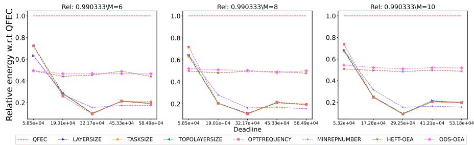
Figure 2516: Assessing the performance of different processor number on the SoyKB workflow.
