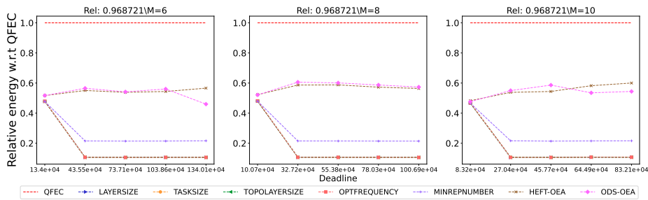
Figure 2935: Assessing the performance of different processor number on the BLAST workflow.
