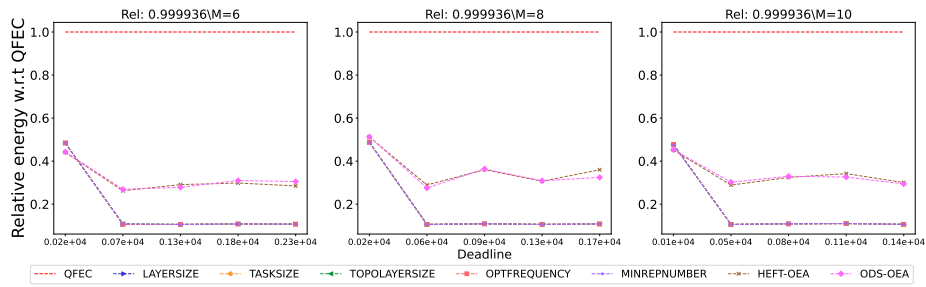
Figure 2713: Assessing the performance of different processor number on the Seismology workflow.
