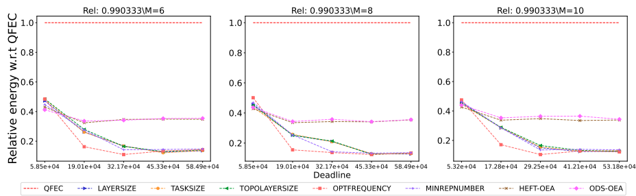
Figure 2681: Assessing the performance of different processor number on the SoyKB workflow.
