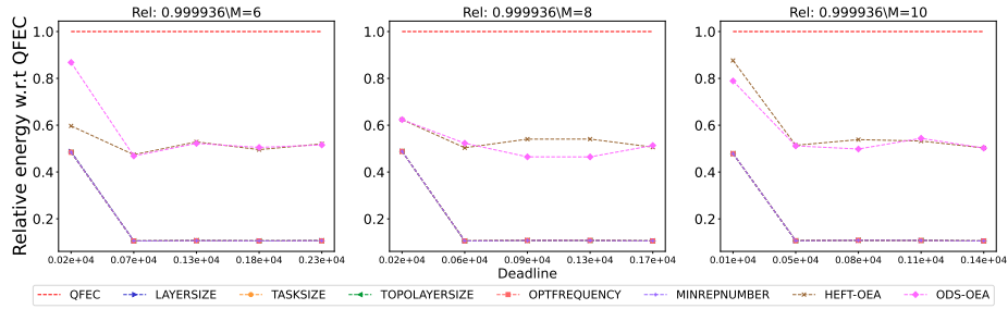
Figure 3021: Assessing the performance of different processor number on the Seismology workflow.
