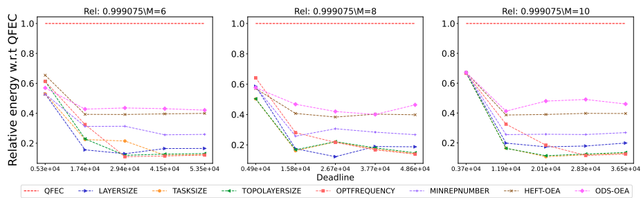
Figure 2774: Assessing the performance of different processor number on the Epigenomics workflow.
