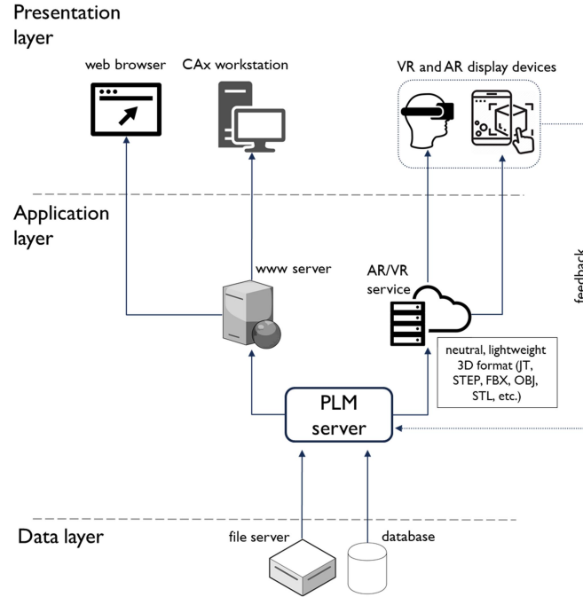
Fig. 3. Generalised architecture of the PLM system integrated with the service performing tasks related to VR and AR technologies
