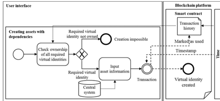
Fig. 3. Model to create virtual identities for assets with dependencies
