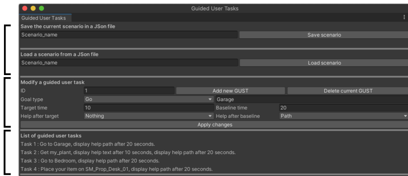
Fig. 9. This interface allows designers to define GUTasks , add and edit task constraints, view the list of existing tasks. The tasks can be easily loaded and exported in the GUsT-3D representation for reuse in various scenarios.
