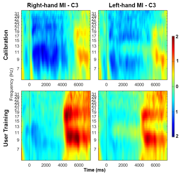
Fig. 3: Grand average time-frequency analysis ( n=70 ) with event-related spectral perturbation (ERSP) for both Calibration and User Training sessions for electrode C_3 . t=0 on this plot corresponds to t=3 on the trial showed in Figure 1
