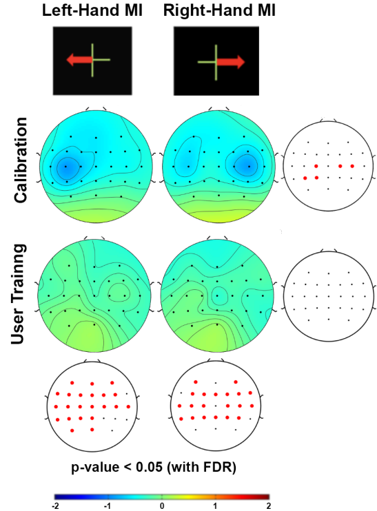
Fig. 2: Topographic map of ERD/ERS% (grand average, n=70 ) in the alpha/mu+beta band during the right-hand and left-hand MIs for both calibration and user training sessions. A blue colour corresponds to a strong ERD and a red one to a strong ERS. Red electrodes indicate a significant difference ( p < 0.05 ) with a FDR (False Discovery Rate) correction.
