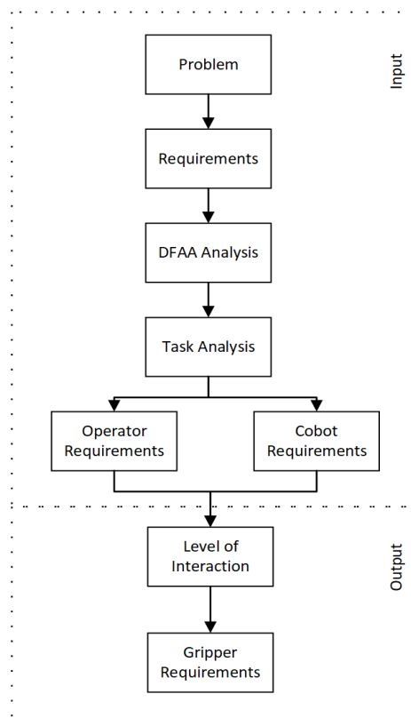
Figure 2: Framework for identifying gripper requirements
