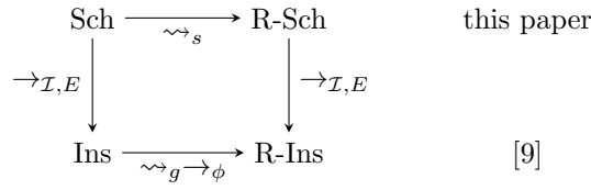
Figure 12: Schema of the proof of correctness.
