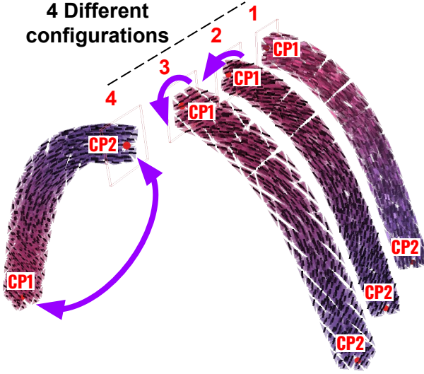
Fig. 2: QP simulation with 4 configurations of a simple beam subject to only gravity. Purple arrows represent the new change in the configuration compared to the first (1). Configuration 2 & 3 have two different rotation around their longitudinal axis and for 4 the tip and attached part were switched.
