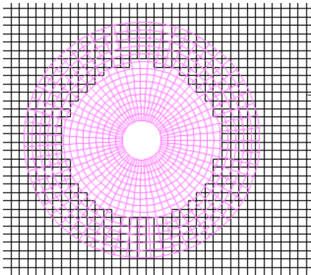
Fig. 1: Example of Chimera grid configuration. In black there is the background mesh and in pink the foreground mesh.
