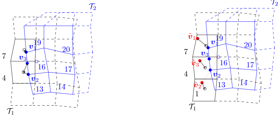
(b) Second step: by identifying the symmetric points \tilde{v}_\mu , \mu = 1, 2, 3 , (red full dots) of the node of the cell \Omega_{16} (blue empty dot) with respect to the vertexes and the middle point of the not shared edge, look for the nodes of cells in the partition \mathcal{T}_1 minimizing the Euclidean distance to those points.
