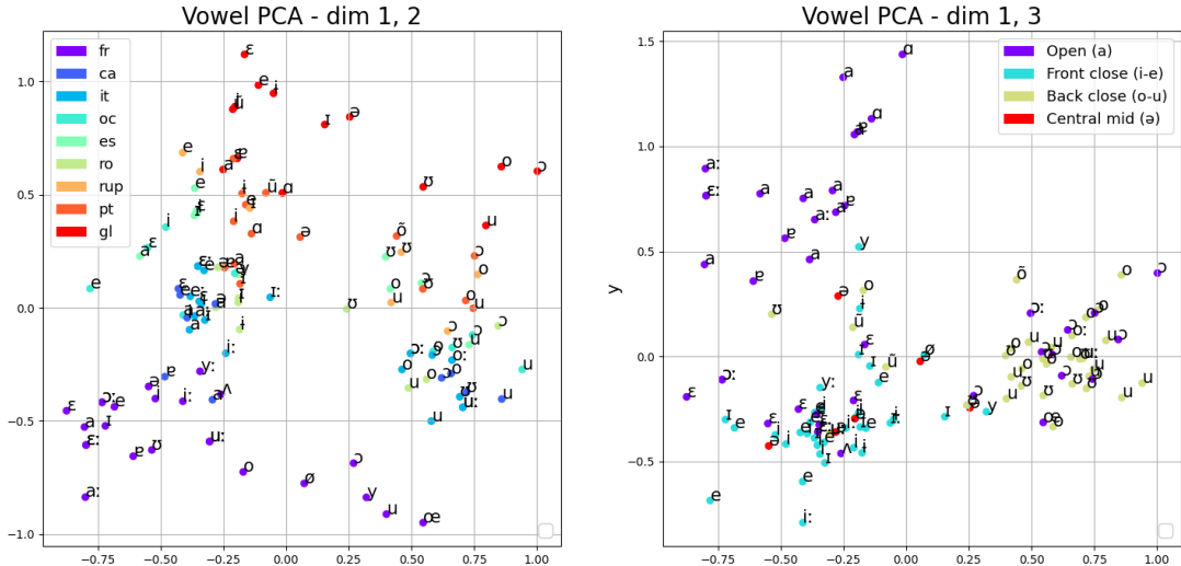
Figure 4: Vowels PCA, seed 0. Left: coloured on language. Right: coloured on pole of the vocalic triangle
