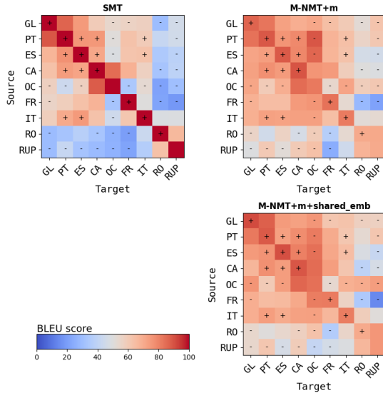
Figure 3: Heatmap of the BLEU scores for our models of interest.
