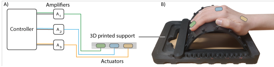
Fig. 1. Experimental set-up. A) The signals are generated via a controller and then amplified before being played by the custom-built actuators. B) Three electromagnetic actuators are placed on a curved hand-rest. The colored dots show the contact points of the actuators on the hand.
