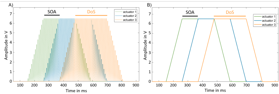
Fig. 2. Signals sent to the three actuators in the two actuation modes. A) Vibratory mode, made of sinusoidal oscillations at 120 Hz within ramp envelopes. B) “Tap” mode made of single ramp signals. In this Figure, we used \text{DoS} = 220 ms and \text{SOA} = 110 ms.
