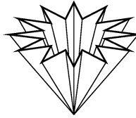
Fig. 1: Example of pathological vertex (cf. [10, §5])
