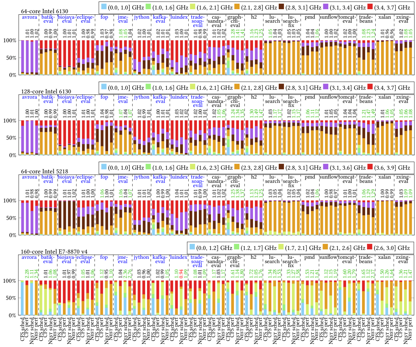
Figure 11. DaCapo tests, frequency distribution. The numbers above the bars indicate the speedup as compared to CFS-schedutil. Red numbers indicate a degradation of more than 5%. Green numbers indicate a speedup of more than 5%.
