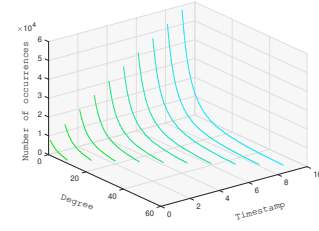
Figure 6: Zipfian degree distribution of a growth only graph
