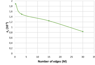
Figure 11: \varepsilon_c in function of the number of edges.
