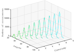
Figure 4: Gaussian degree distribution of a growth only graph
