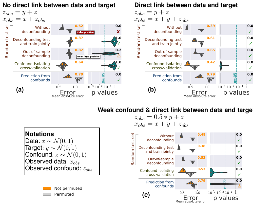
Figure 8: Benchmarking approaches to control confounded predictions on simulated data with many samples. The left column of each subfigure assesses the prediction performance through the mean absolute error (in signal units). We display the error distribution across validation folds for the data (top, orange) and for permuted data distribution (bottom, gray). The right column displays the distribution of P-values across folds, obtained by permutation, and the text reports the aggregated P-value across folds (see main text). Five approaches are benchmarked: without deconfounding, deconfounding test and train jointly, out-of-sampling deconfounding, confound-isolating cross-validation, and prediction from confounds. There are 3 simulation settings: (a) no direct link between target and brain, (b) a direct link between target and brain, and (c) a weak confound and a direct link between target and brain. Green ticks indicate correct conclusions, red crosses mark incorrect ones, and warning signs, the weak results.
