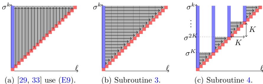
Fig. E5: Comparison of the computation load of (E9) used in [29, 33] with the one of Subroutine 3 and Subroutine 4.
