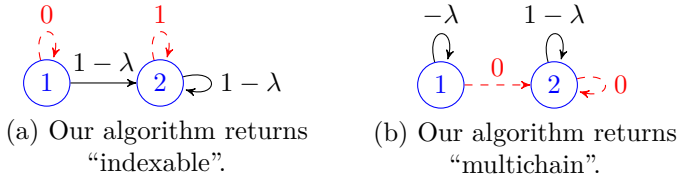
Fig. A3: Example of an indexable multichain problem with infinite Whittle index. Transitions are deterministic and labels on edges indicate rewards (for the \lambda -penalized arm). Solid black transitions correspond to action "activate" and dashed red to the action "rest".
