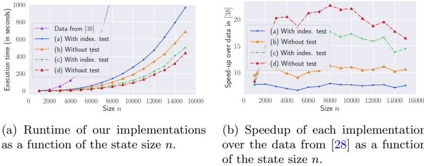
Fig. 5: Numerical result over 7 simulations taking around 21 hours in total: in each simulation, we run the algorithm over randomly generated RBs with the state size ranging over \{1000, \dots, 15000\} . We plot the average runtime over 7 simulations. The solid lines represent the result of Subroutine 3 and the dashed-dot lines represent the one of Subroutine 4. The marker “+” indicates that algorithms test indexability and the triangles indicates that algorithms do not test indexability.
