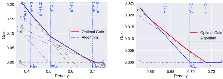
(a) Overview of the visited \mu_{\min}^k . (b) Zoom on \lambda \in [0.65, 0.73]
