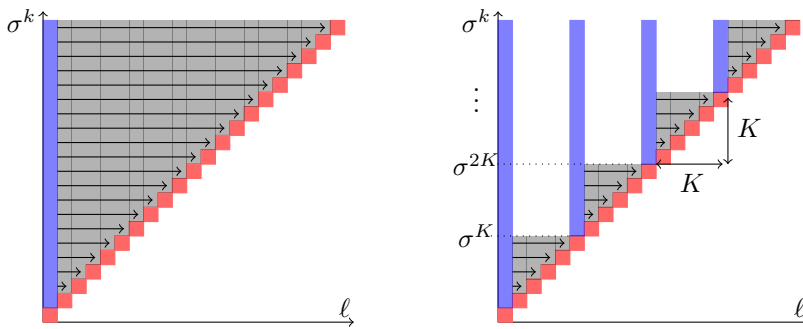
(a) Implementation of Subroutine 3. (b) Implementation of Subroutine 4
