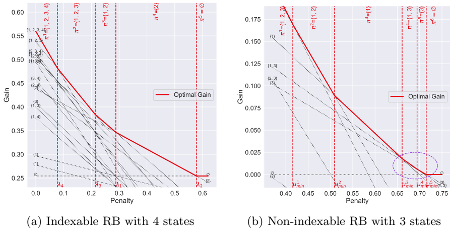
Fig. 1: The average gain as a function of penalty for two examples, one which is indexable (Figure 1a) and the other one which is not (Figure 1b).
