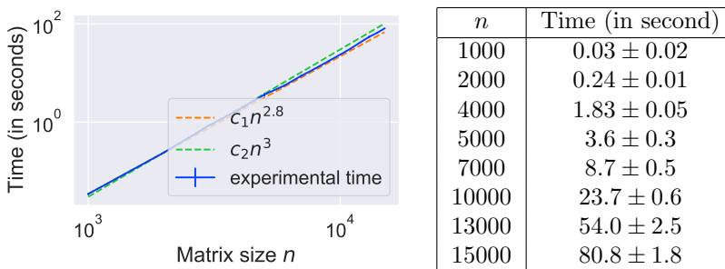
Fig. C1: Time taken of the default implementations scipy.linalg.solve of scipy to solve a linear system \mathbf{AX} = \mathbf{B} where \mathbf{A} and \mathbf{B} are two square n \times n matrices.
