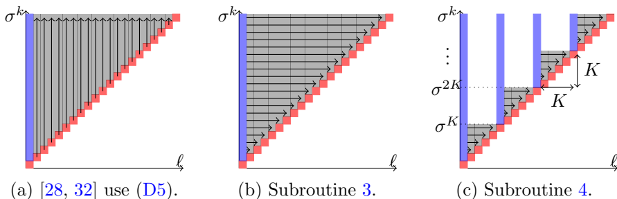
Fig. D2: Comparison of the implementation of (D5) used in [28, 44] with Subroutine 3 and Subroutine 4.
