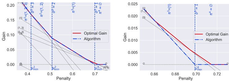
(a) Overview of the visited \mu_{\min}^k .
