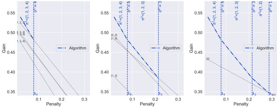
(a) After the 1st iteration. (b) After the 2nd iteration. (c) After the 3rd iteration.
