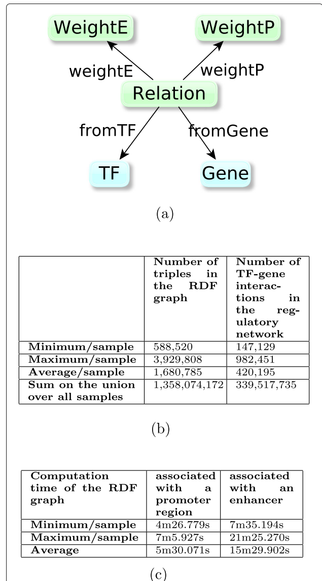
Fig. 4 a RDF-model for each sample-specific graph: boxes represent classes of entities; a relation between a TF and a gene is characterized by (i) WeightP , the score which models the ability of the regulation to be operated through a promoter region, and (ii) WeightE , the score which models the ability of the regulation to be operated through an enhancer region. At least one of these scores has a nonzero value. b Description of the content of the 808 sample TF-gene regulatory networks. Each network is represented by an RDF graph based on the RDF model described in (a). The number of TF-gene interactions in the corresponding regulatory network is the number of instances of the "Relation" class in the graph. c Execution times of the SPARQL queries Insert_Enhancer.rq and Insert_Promoter.rq (cf. Fig. 2 and github repository) for constructing the graphs in (b), calculated for the first 102 samples. Structure of the 808 sample-specific graphs representing the parameters of the TF-gene regulation relations
