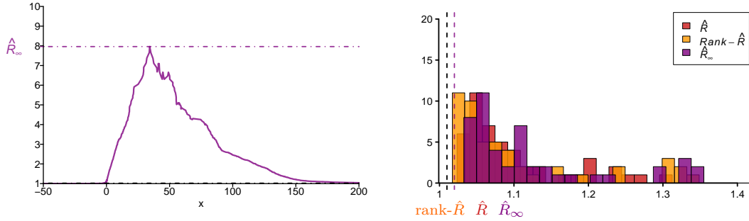
Example 7.b: HMC on alternative Cauchy
