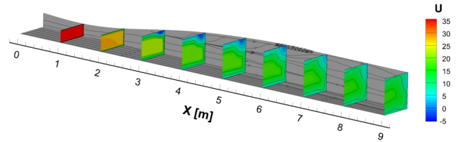
Figure 10: Flow topology for the Spalart-Allmaras QCR model. The lines indicate the skin friction direction.
