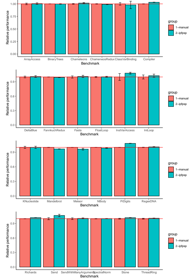
Figure 7: Manual vs Automatic Localization of IP, FP and SP. Average of 100 iterations, error bars show standard deviation. Results are relative to no localization. Higher is better.
