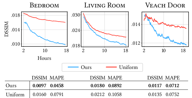
Fig. 13. Quantitative evaluation of our method and ablations compared to ground truth (graphs start at 2h of training.)
