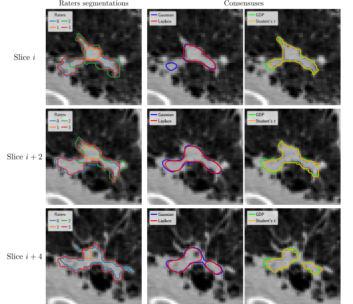
Fig. 9. Comparison of the heavy-tailed distributions on a nodule segmentation case extracted from the NoduleBin dataset.
