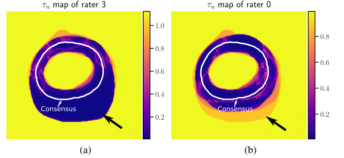
Fig. 6. The outlier, rater 3, exhibits locally poor performances linked to lower values of \tau_n^p , in particular at the bottom of the image in the region indicated by the black arrow (6a). In contrast, rater 0 shows higher \tau_n^p values in the same area (6b).
