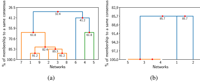
Fig. 17. Complete-linkage clustering of the networks based on the percentage of membership of the same consensus for the NoduleNet (17a) and ProstateNet (17b) datasets.
