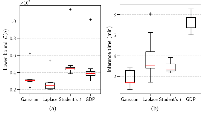
Fig. 11. Lower bound values reached after convergence (11a) and computation times obtained on the 20 nodules from NoduleBin dataset (11b).
