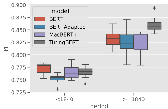
Figure 4: Evaluation in terms of F1-score on the HIPE2022 dataset for Named Entity Recognition in English. Results are split into an earlier and a later period taking 1840 as the median date of the texts in the dataset.
