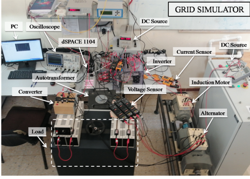
Figure 1. Grid voltage emulator setup [36].
