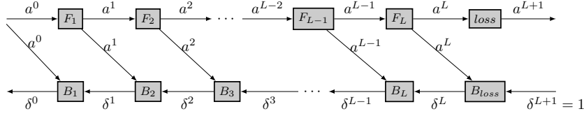
Figure 1: Data dependencies induced by the training phase of Sequential DNNs
