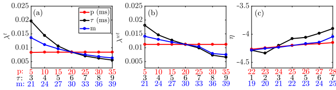
Fig. 6. Panels a–c: Sensitivity of \lambda^t (left), \lambda^{wt} (middle) and \eta (right) for different values of the parameters representing the period ( p ), delay ( \tau ) and embedding dimension ( m ) calculated from unwarped and warped T waves in a 2-minute window and inter-MWTW of a patient at a particular HD stage ( h_4 ). Note that the default values of p , \tau and m used in the calculation of \lambda^t and \lambda^{wt} are different from the ones used in the calculation of \eta , which explains differences in the x-axis of panels (a) and (b) with respect to panel (c).
