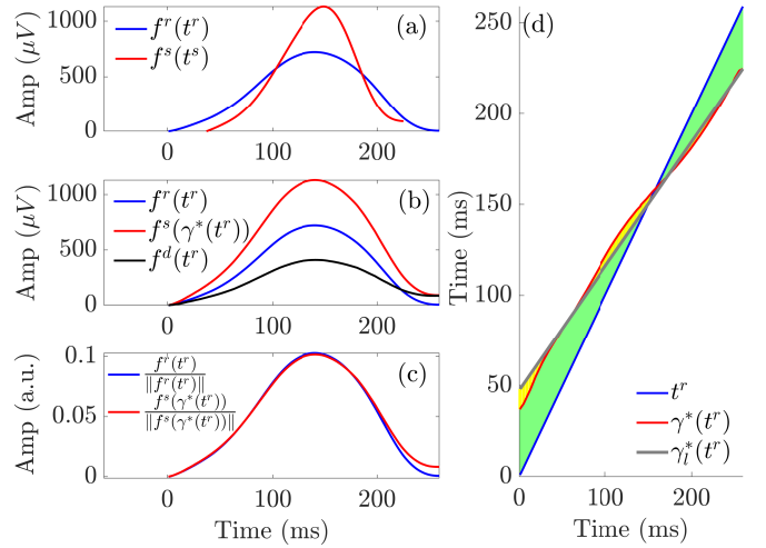
Fig. 3. Time-warping analysis for one ECG recording. Panel (a) shows reference (blue) and investigated (red) T waves obtained from an ECG segment during HD. Panel (b) shows the warped T waves, which have the same duration while keeping the original amplitude, and the difference between them (black). Panel (c) shows the warped T waves after normalization by their L^2 norms. In panel (d), the green area between the blue line and the red curve represents d_w , which quantifies the total amount of warping in the time domain. The dark gray solid line is the linear regression function \gamma_l^*(\mathbf{t}^r) best fitted to \gamma^*(\mathbf{t}^r) .
