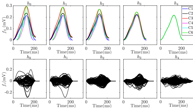
Fig. 7. Simulated (last) T wave from a sequence of 2 minute T waves ( f_S^k ) in linear and nonlinear duration and amplitude domain (top panels) and the variability ( f_v^k ) in 2 minute T waves (bottom panels) during HD. Solid black and red T waves correspond to nonlinear and linear amplitude modulation (C2, C3), solid cyan and magenta T waves correspond to nonlinear and linear duration modulation (C4, C5), and solid green T wave includes both time and amplitude modulation (C6). Blue T wave corresponds to the reference T wave (C1).
