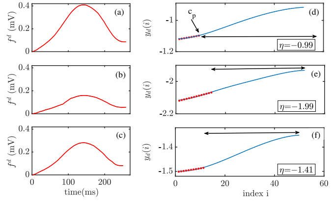
Fig. 5. Panels a–c: Inter-MWTWs from a particular patient at different HD stages ( h_0, h_1, h_{48} ). Panels d–f: y_d(i) computed as described in the text, with indication of the corresponding \eta values.
