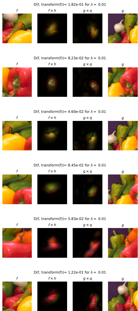
Figure 6: \widehat{D}_\lambda(f, \text{transform}(f)) for f random patches from peppers . We show f , g = \text{transform}(f) as well as the optimal functions h and q .
