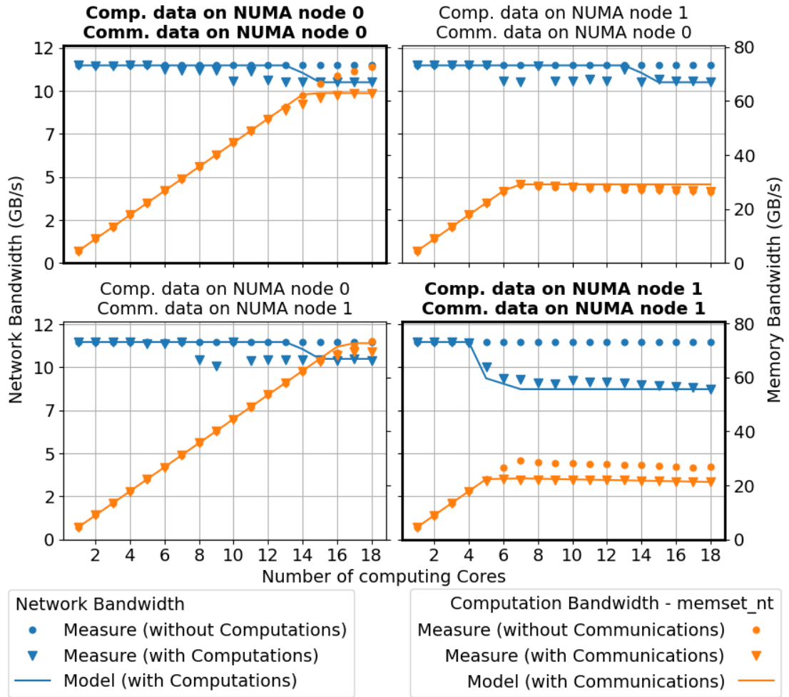
Figure 3: Performances of computations and communications along with our model prediction on henri (INTEL, INFINIBAND).
