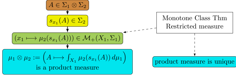
Figure 2: Flowchart for the construction of the product measure. The fill colors refer to sections: 4.1 in brown, 4.2 in yellow, 4.3 in green, and 4.4 in blue. Dashed lines denote the use of the listed proof arguments, that were developed for the present work.
