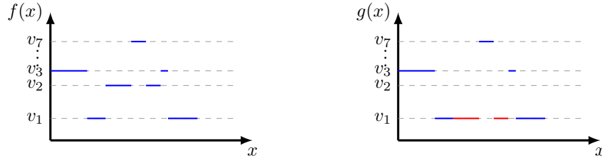
Figure 1: Illustration of Lemma SF_aux_cons . The value v_2 taken by the simple function f (on the left) is replaced in g (on the right) by the value v_1 (in red).
