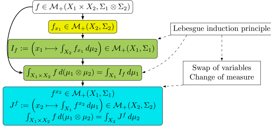
Figure 4: Flowchart for the construction of the iterated integrals on a product space. The fill colors refer to sections: 5.1 in yellow, 5.2 in green, and 5.3 in blue. Dashed lines denote the use of the listed proof arguments, that were developed for the present work.
