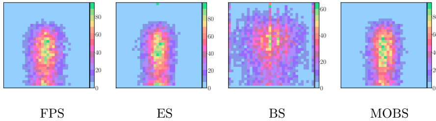
Figure 3: Behavioral Maps with 32 \times 32 bins. x -axis represent the item type ratio (leftmost bins represent behaviors that collect only black items, those that collect equally are in the middle, and those that collect only red are on the right) the y -axis represent the maximum traveled distance (zero distance at the topmost, maximum distance at the bottom). Maps aggregate behaviors from the last 10 generations.
