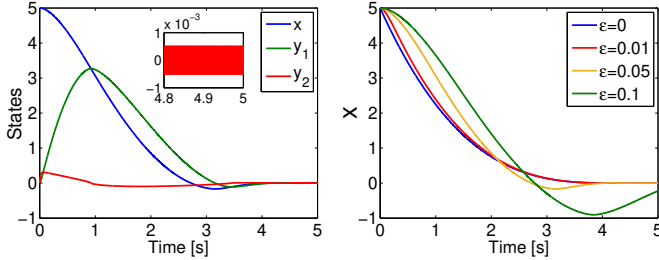
Fig. 2: On the left: behavior of the closed-loop system (48)-(49) where \alpha = 1.2 and \epsilon = 0.05 . On the right: comparison of the deviation of the state of the plant for different values of the parameter \epsilon .
