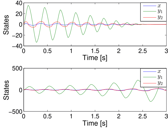
Figure 5: Behavior of the closed-loop systems (54)-(55) where \alpha = 60 , \epsilon = 0.01 , x_0 = 2 and y_0 = [0, 0] (top), or x_0 = 5 and y_0 = [0, 0] (bottom).
