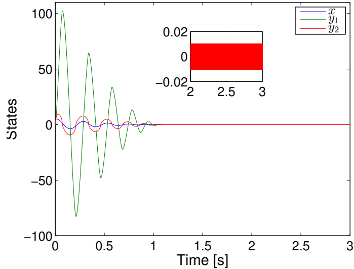
Figure 6: Behavior of the closed-loop systems (54)-(55) where \alpha = 60 , \epsilon = 0.005 , x_0 = 5 and y_0 = [0, 0] .
