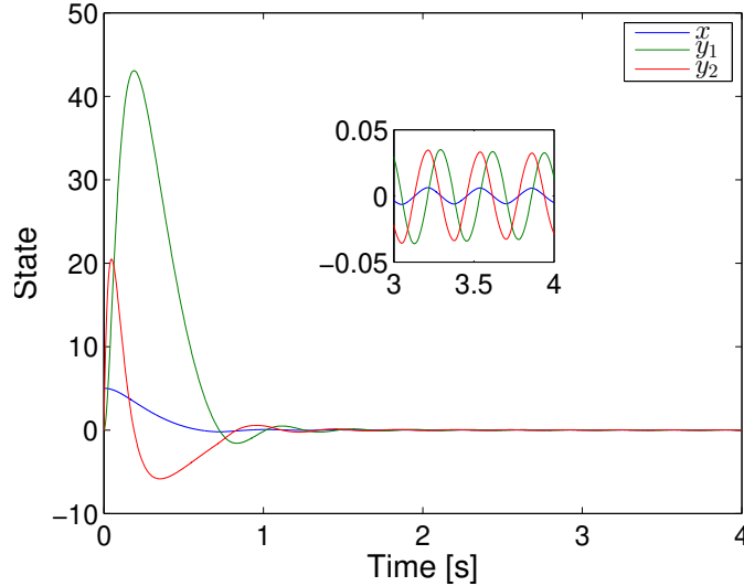
Figure 1: Behavior of the interconnected system (47)-(48) where \alpha = 5 and \epsilon = 0.05 .
