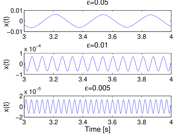
Figure 2: Chattering in the output of the closed-loop system (47)-(48) with \alpha = 5 .
