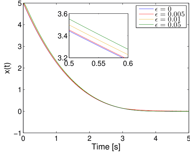
Figure 4: Comparison of the behavior of the closed-loop system (51)-(52) for different values of \epsilon .
