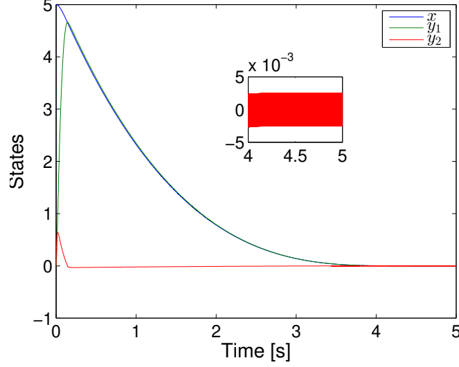
Figure 3: Behavior of the closed-loop system (51)-(52) where \alpha = 1.2 and \epsilon = 0.01 .
