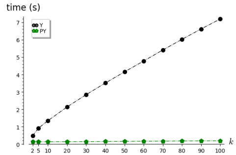
(a) Average running time on Stockholm
