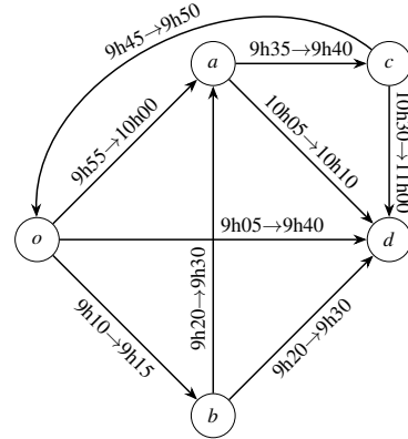
Figure 1: Toy network for k earliest arrival time journeys reaching d , departing after t_0 and arriving before t_{max} .
