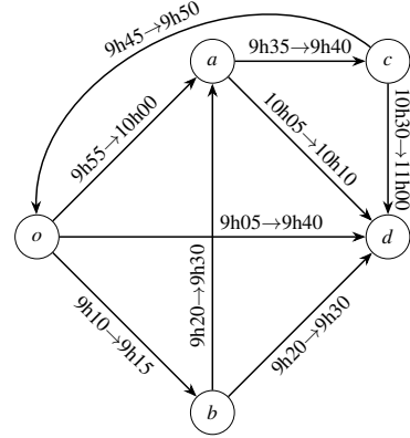
Figure 1: Toy network for k earliest arrival time journeys
