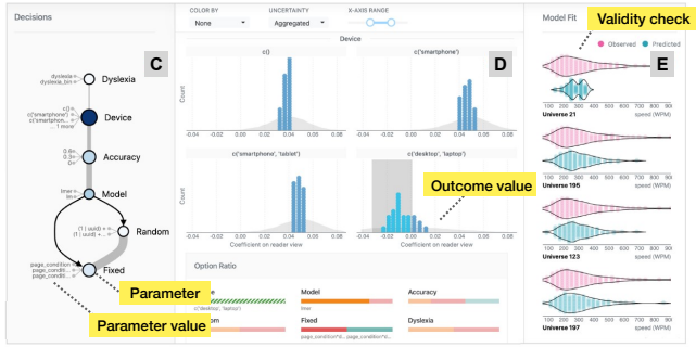
Figure 15: Screenshot of the Boba system [LKAH20]. Panel C shows the design space of parameters and their relationships; parameters that are source of sensitivity are in a darker color. Panel D is a trellis of dotplots of outcome values, subsetted by parameter values. Panel E shows predictive distributions from each universe compared to the observed data.
