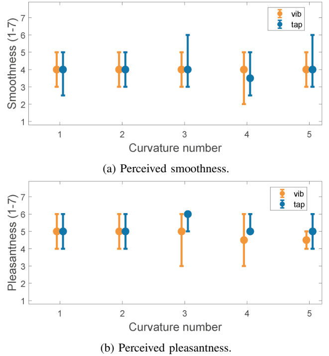
Fig. 6: Rates on a 7-point Likert scale for the AHM. The smoothness was rated after each trial of the experiment and each data point is averaged over an experimental block. The middle points correspond to the median value while the error-bars give the 1st and 3rd quartile. Same plot was made for the pleasantness.
