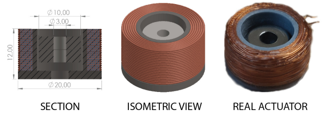
Fig. 2: CAD and picture of the custom electromagnetic actuators. The coil structure (dark grey) is 3D printed, and two magnets (light grey) glued in their repulsive position constitute the mover. The designed is inspired by Duvernoy [18]. Dimensions are in mm.
