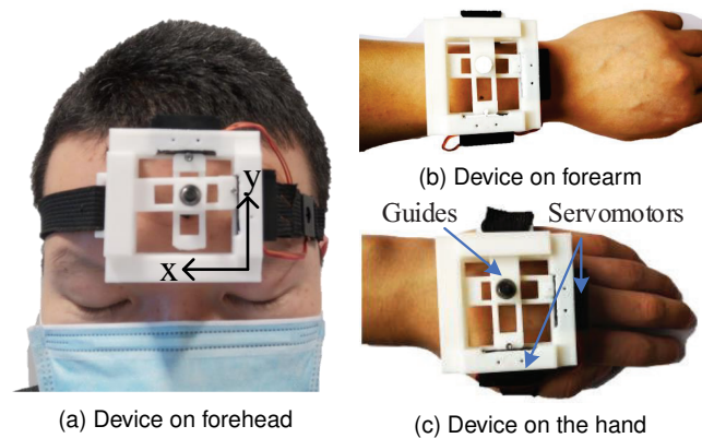
Fig. 3. The prototype of our wearable cutaneous device worn on the (a) forehead, (b) forearm, and (c) back of the hand.
