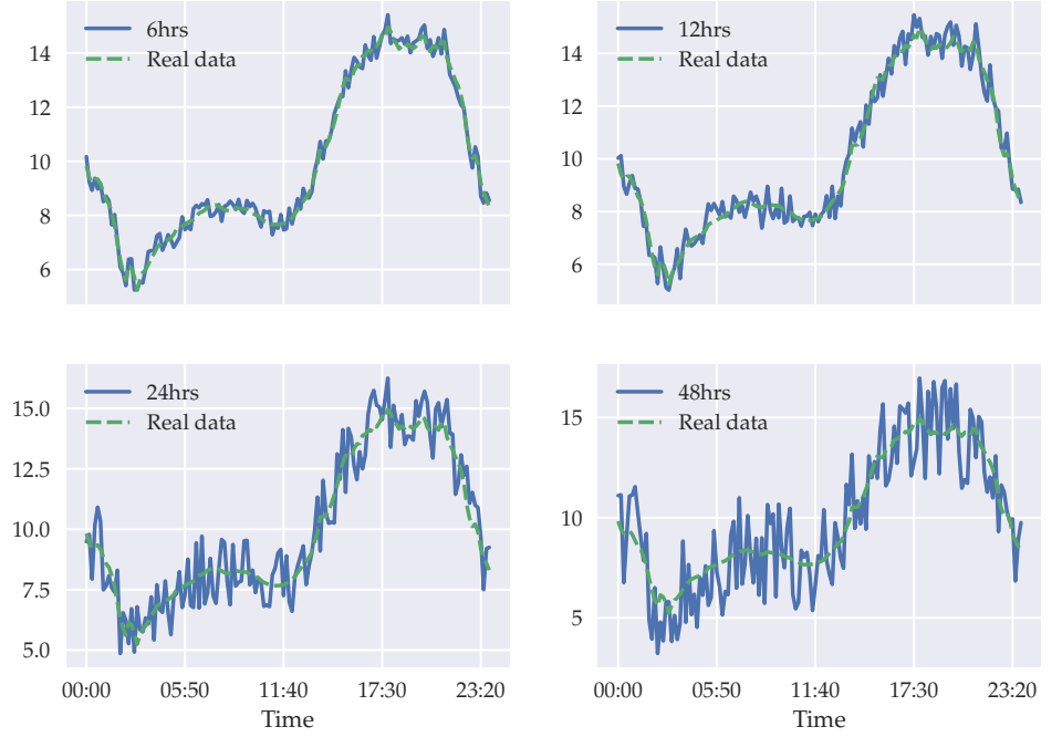
Figure 8. GRAFT-Frost model results compared with real data for 6, 12, 24 and 48 hours forecasts.
