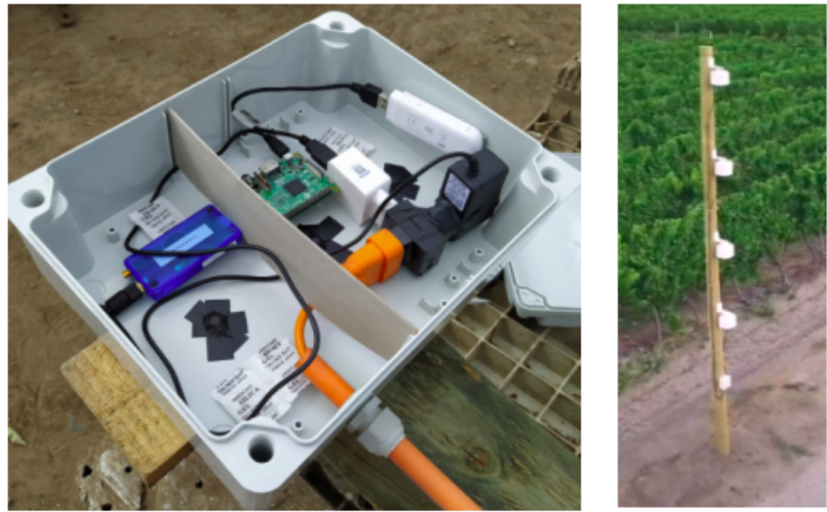
Figure 2. IoT platform installed on the experimental field composed by temperature and humidity sensors.
