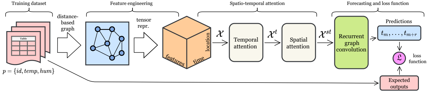
Figure 3. Overview of the GRAFT-Frost model.
