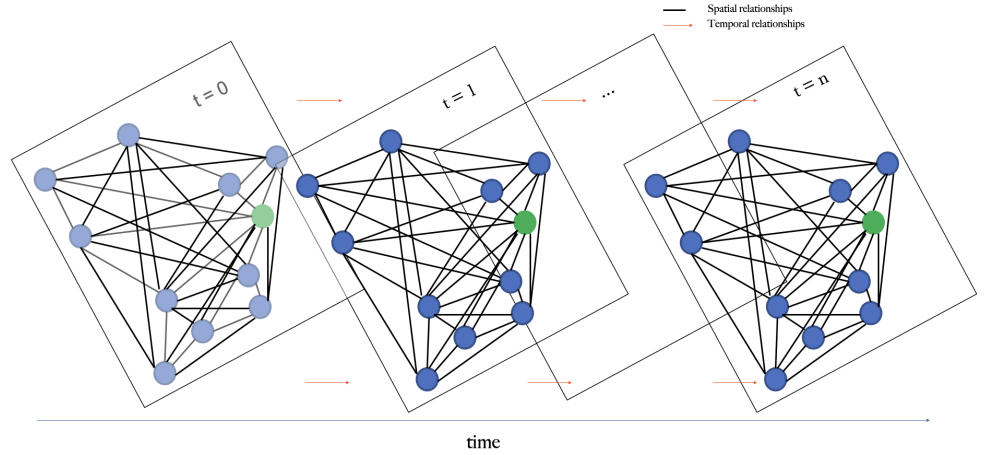
Figure 4. Schematic view of the spatio-temporal graph network for modeling the relationships between the experimental field and weather stations through time.
