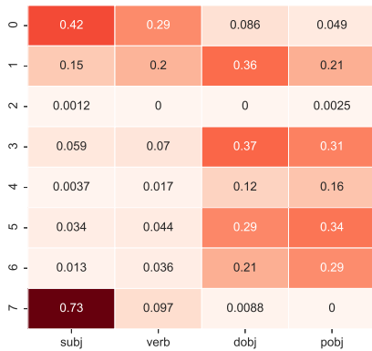
Figure 6: Encoder influence heatmap for \text{Yelp}(\Gamma^{enc}) .
