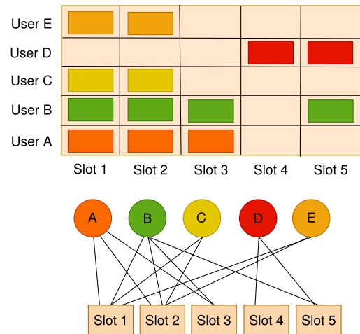
FIGURE 1. IRSA representation: transmissions of users in slots (top), coding theory representation to model the decoding process (Tanner graph, bottom). Note that transmissions are in the same frequency channel, hence when two users are transmitting on the same slot, there is a collision.
