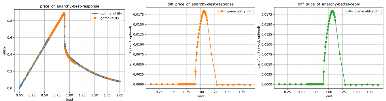
(b) The Price of Anarchy (difference with optimal) for the best response strategy
