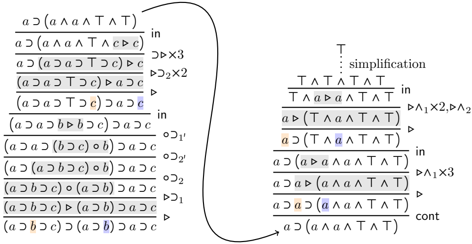
Figure 3. Lnip derivation fragment for the S-combinator
