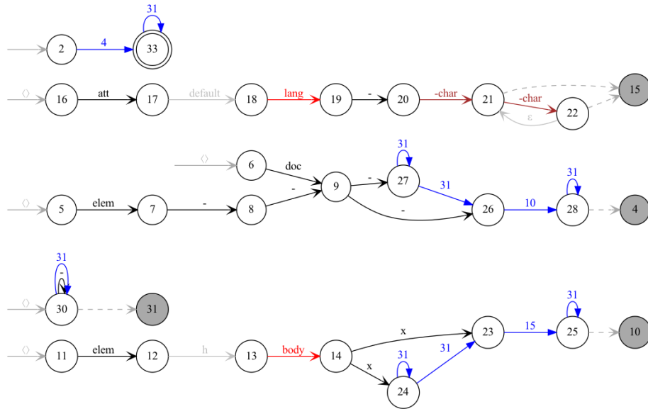
Fig. 2: The nondeterministic SHA A_2 = sha(Q_2) .
