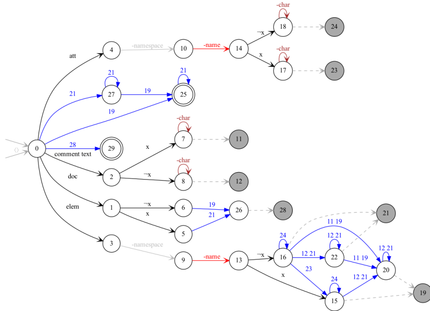
Fig. 1: The dSHA xml\&one^x : a schema for x -annotated XML documents.
