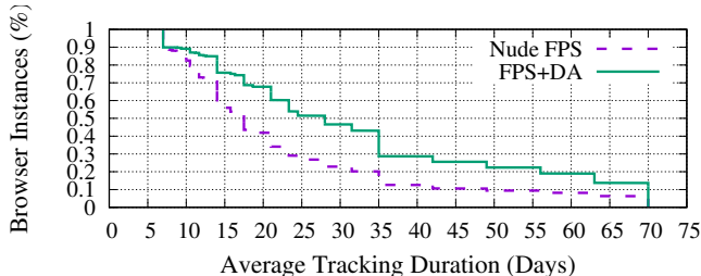
Fig. 6. Differences in Average Tracking Time between FP-STALKER (Nude FPS) and FP-STALKER with DRAWNPART (FPS+DA)
