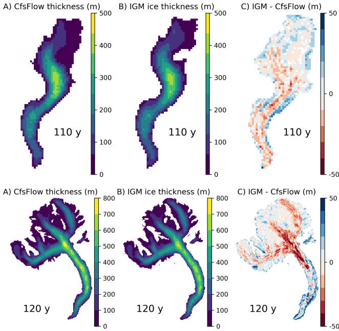
Figure 13: Ice thickness fields of Rhone (top panels) and Aletsch (bottom panels) glaciers after 110 and 120 years with CfsFlow (A) and IGM (B), as well as the difference between the two (C).
