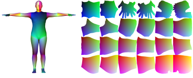
Fig. 2. Illustration of the template geometry IUV mapping.
